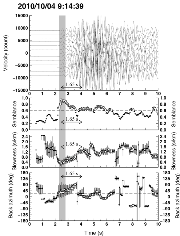
Fig. 5 Time evolution during 10 s of the array analysis results of an explosion earthquake in the 2-4 Hz band. The time displayed at the top corresponds to the start of the array data. The solutions with semblance values greater than or equal to 0.6 are shown with open circles and the others with smaller solid circles. Vertical lines with circles indicate the uncertainties of the solutions. The dashed line in the semblance panel is the 0.6 threshold. The horizontal dashed line in the back azimuth panel represents the geometrical array-crater direction. The vertical gray band indicates the solutions in the S-wave time window. The double-headed arrows show the time difference between S wave and surface wave arrivals.
