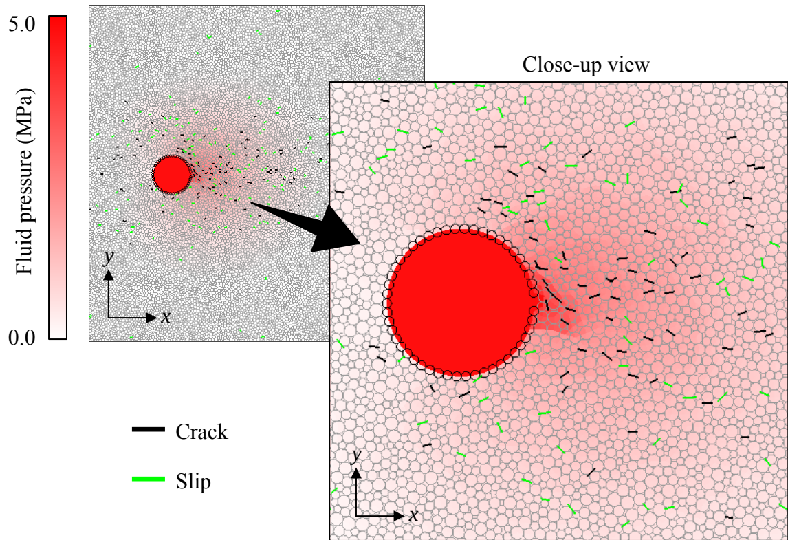
Fig.6.16 Spatial distribution of fluid pressure and micro crack generation at time step= 2354. ( k = 100 [mD], q = 1 [MPa/ 10^7 steps], \mu = 1 [mPa · s] )
