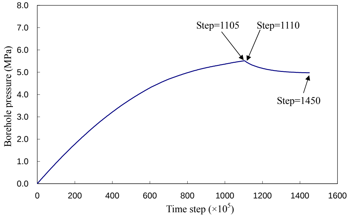
Fig.6.26 Pressure-Time curves. ( k = 100 [mD], q = 1 [MPa/ 10^7 steps], \mu = 2 [mPa \cdot s] )
