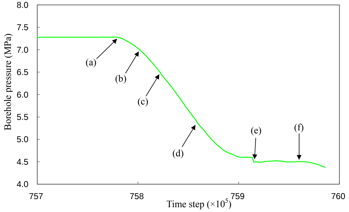
Fig.6.30 Close-up view of the Pressure-Time curve. ( k = 5 [mD], q = 1 [MPa/ 10^7 steps], \mu = 10 [mPa \cdot s] )
