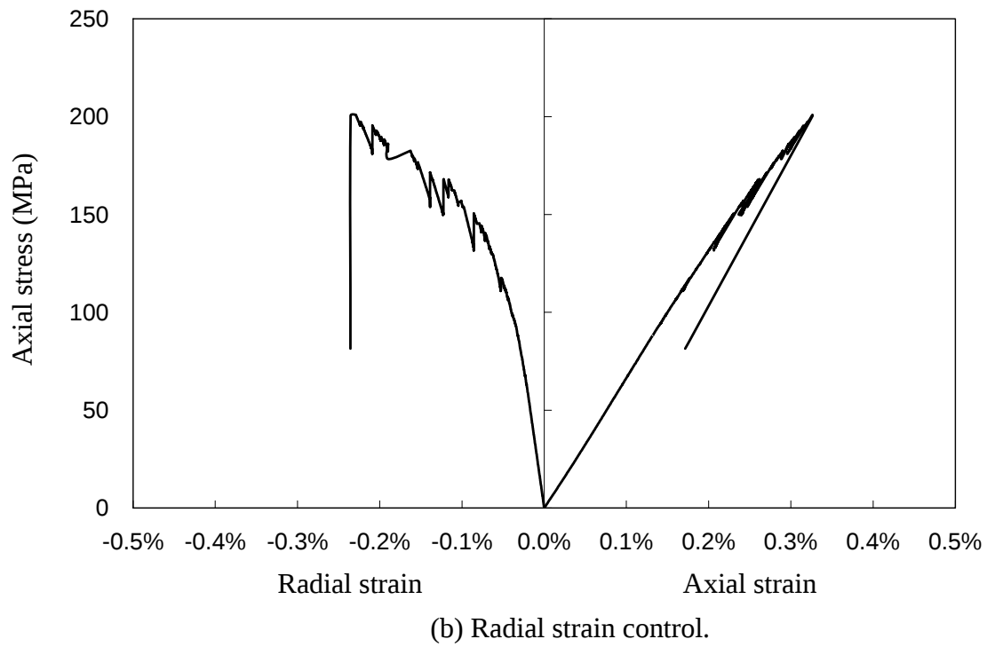
Fig.4.6 Complete stress-strain curves obtained from the simulation with different controlling methods.
