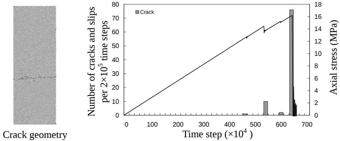
(b) Uniaxial tension test
