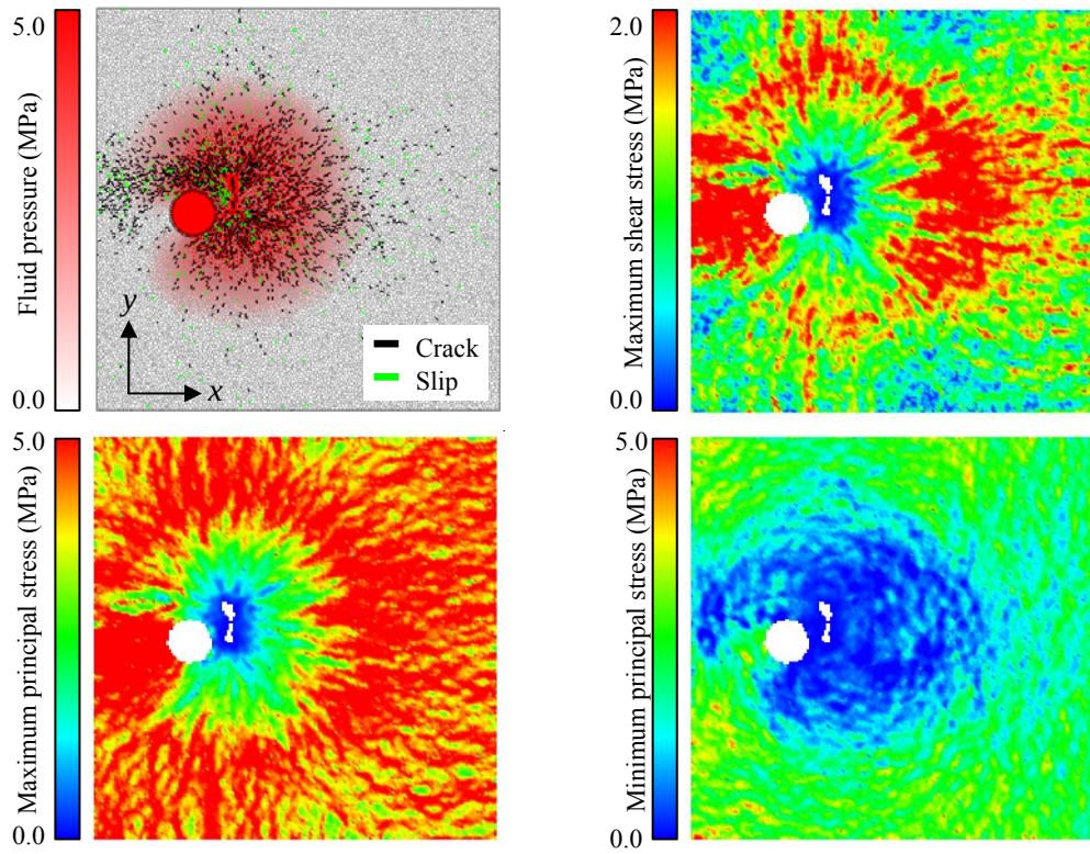
Fig.6.24 Stress state at time step= 594. ( k = 100 [mD], q = 5 [MPa/ 10^7 steps], \mu = 2 [mPa \cdot s] )
