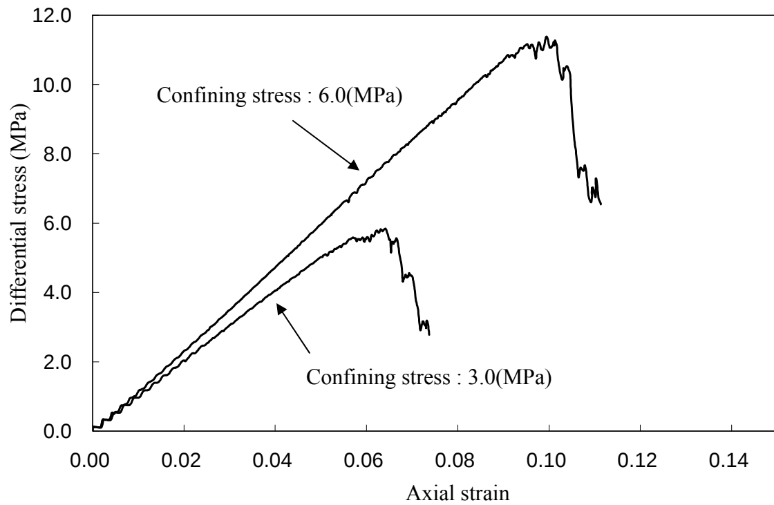
Fig.6.10 Result of the simulation of biaxial compression test.
