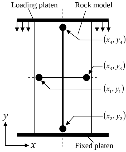
(a) Uniaxial compression test
