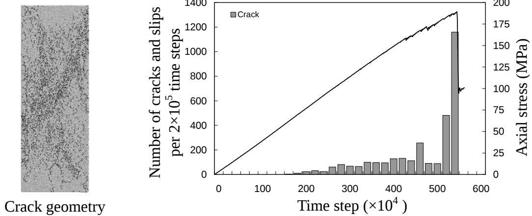
(a) Uniaxial compression test
