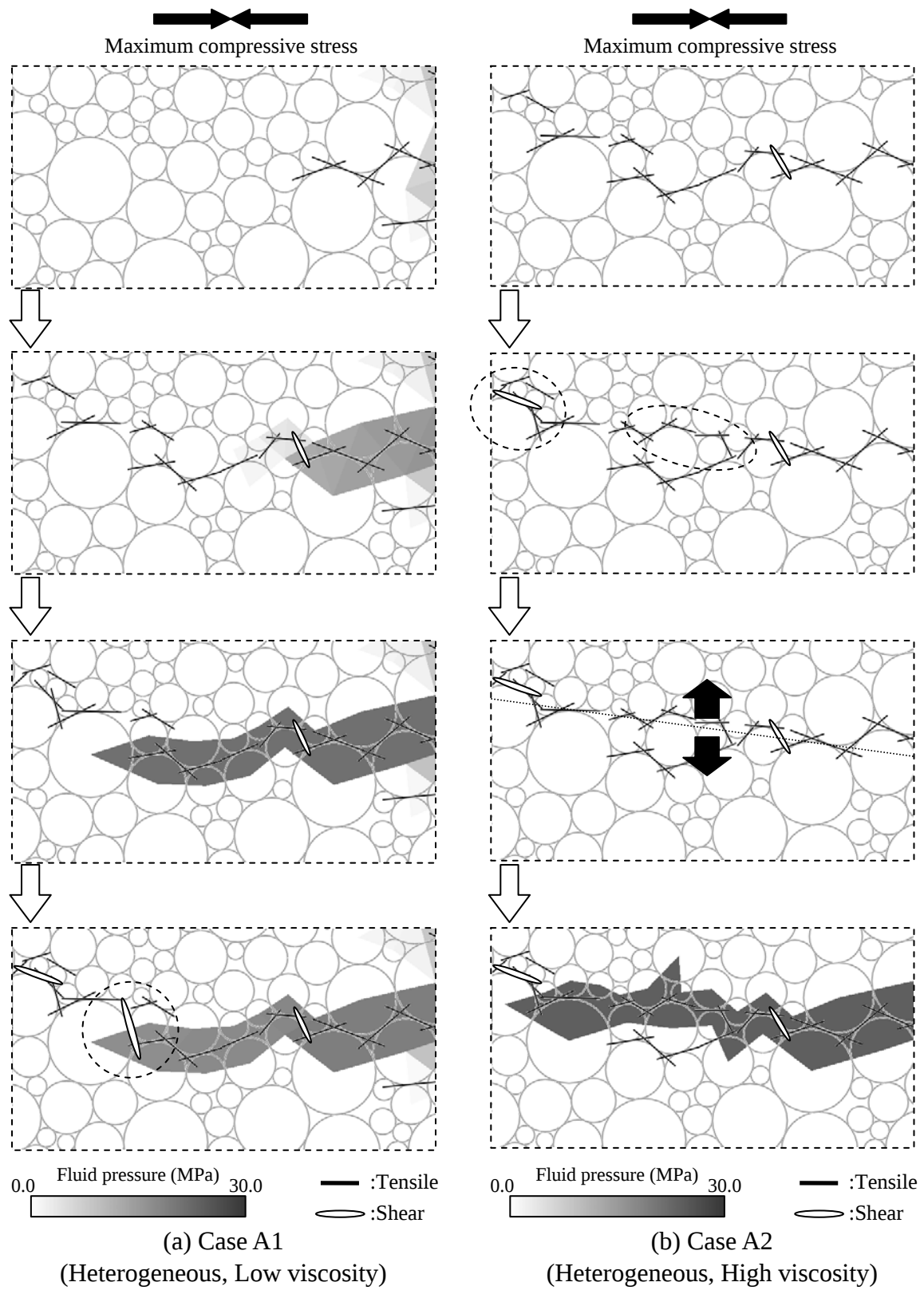
Fig.5.18 Close-up view of the fracture propagation and fluid infiltration behavior.
