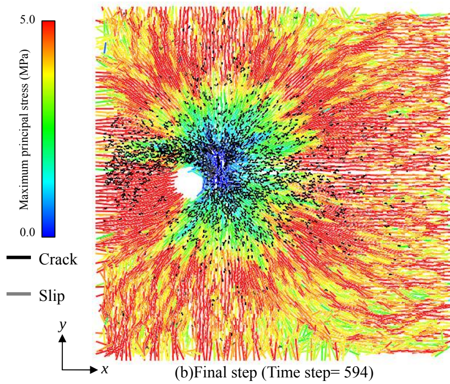
Fig.6.25 Magnitude and direction of the maximum principal stress. ( k = 100 [mD], q = 5 [MPa/ 10^7 steps], \mu = 2 [mPa \cdot s] )
