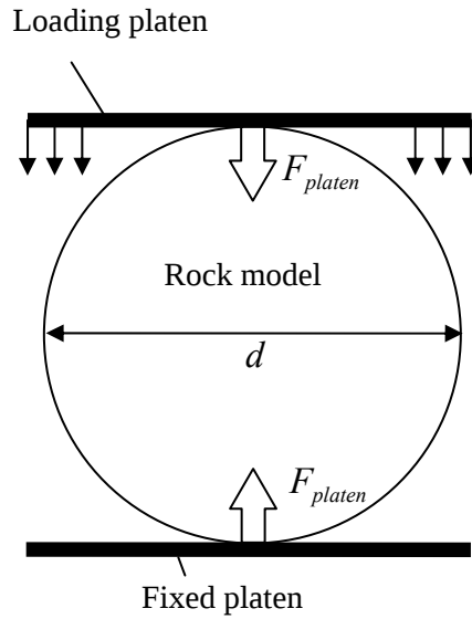
(c) Brazilian test
