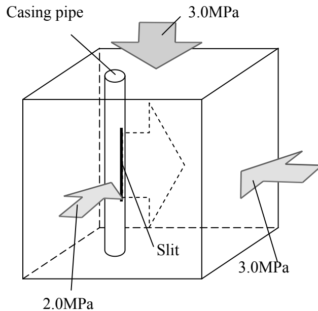
Fig.6.2 Loading condition for the experiment [8,9].
