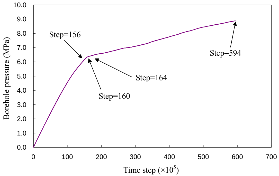
Fig.6.21 Pressure-Time curves.
