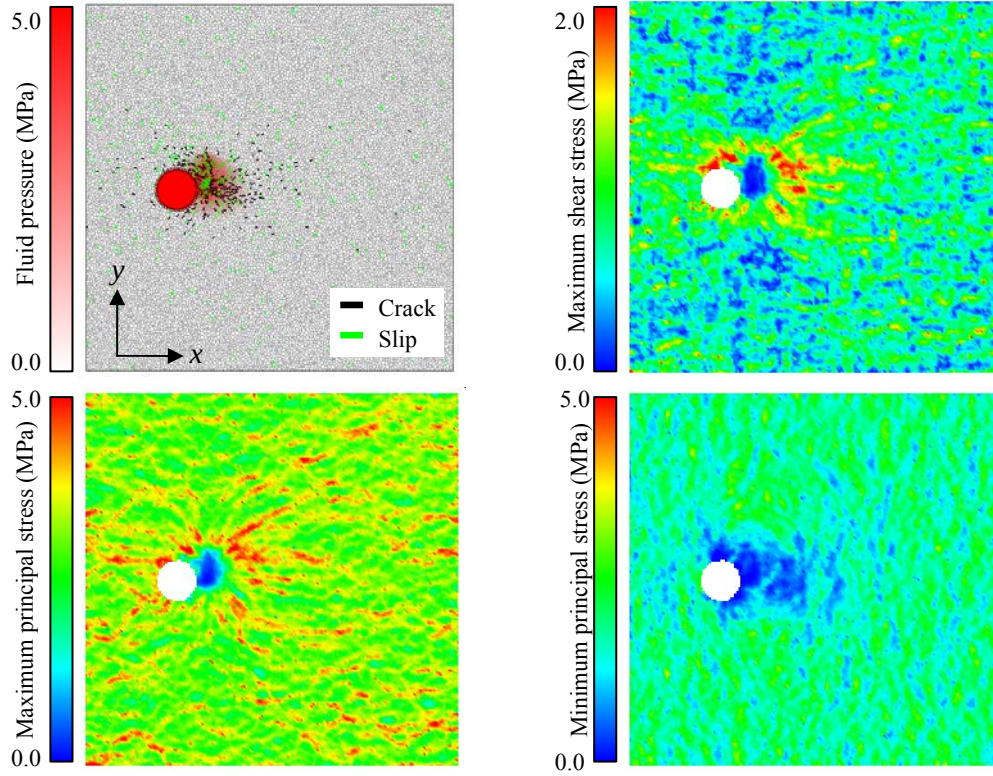
Fig.6.23 Stress state at time step= 164. ( k = 100 [mD], q = 5 [MPa/ 10^7 steps], \mu = 2 [mPa \cdot s] )
