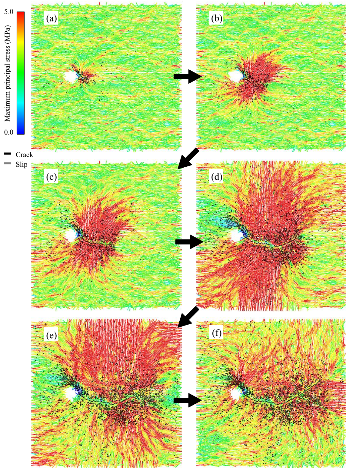
Fig.6.34 Magnitude and direction of the maximum principal stress at each time step. ( k = 5 [mD], q = 1 [MPa/ 10^7 steps], \mu = 10 [mPa \cdot s] )
