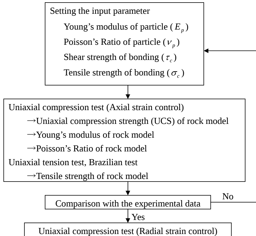
Fig.4.5 Calibration process.
