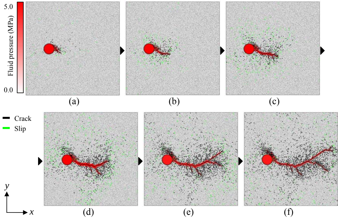
Fig.6.31 Fracture propagation process. ( k = 5 [mD], q = 1 [MPa/ 10^7 steps], \mu = 10 [mPa \cdot s] )
