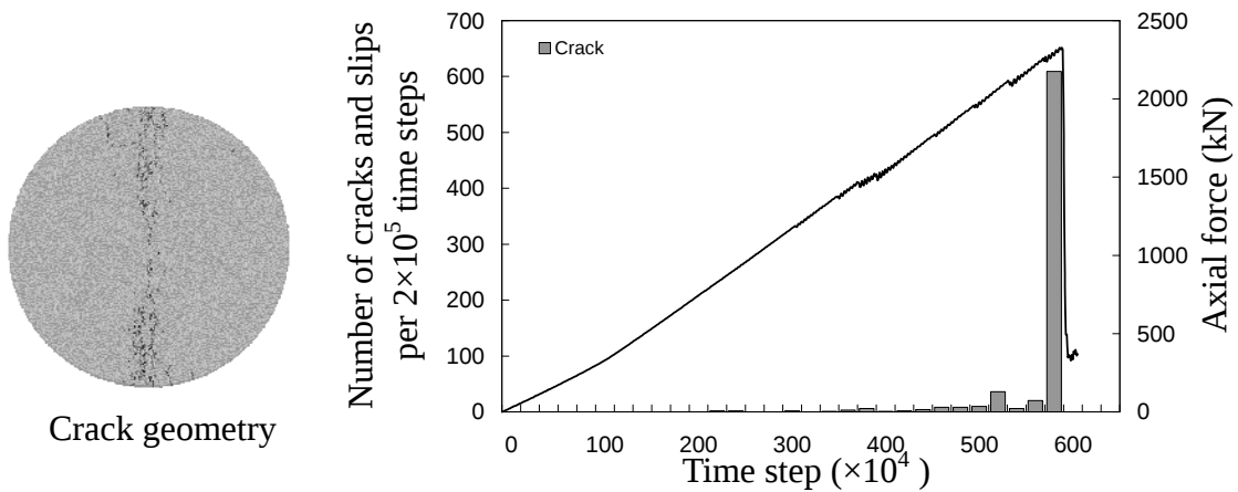
(c) Brazilian test
