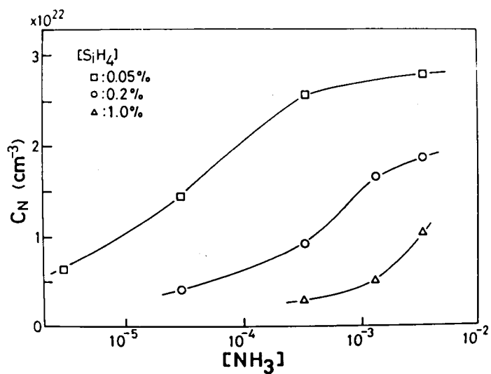
FIGURE 3.4 Incorporated nitrogen content of a-Si:N films evaluated from integrated absorption coefficient.
