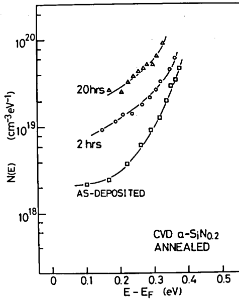
FIGURE 7.4 Field-effect gap-state density in as-deposited, 2-, and 20-h annealed a-SiN 0.2 films.
