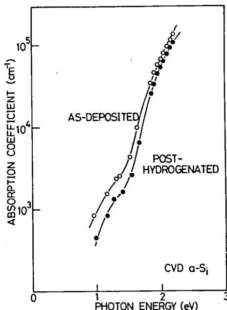
FIGURE 8.1 Absorption coefficient of as-deposited and post-hydrogenated CVD a-Si films.
