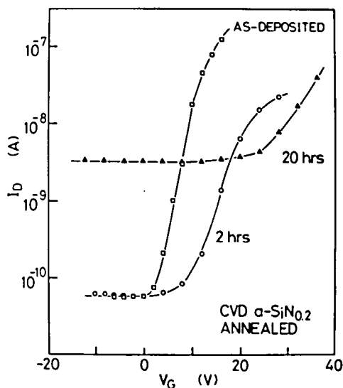
FIGURE 7.3 Field effects of as-deposited, 2-, and 20-h annealed \text{a-SiN}_{0.2} films.
