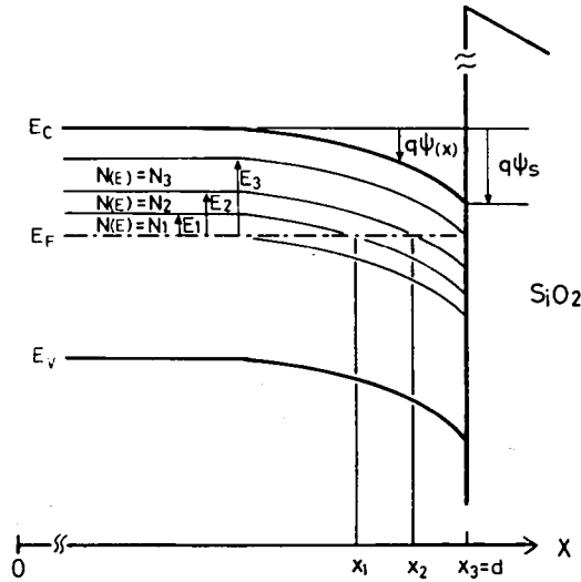
FIGURE 2.5 Definition of x_L in the calculation of source-drain conductance.
