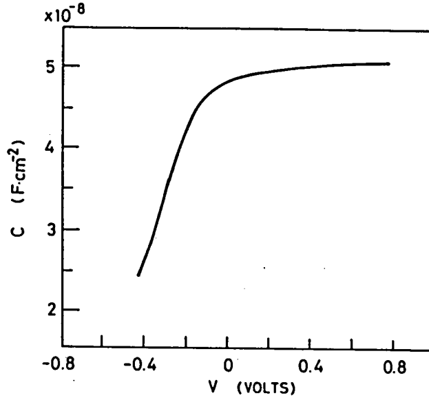
FIGURE A.2 A typical C - V characteristic of CVD a-Si/n-type c-Si ( n_B = 2 \times 10^{15} \text{ cm}^{-3} ) junctions in which the a-Si thickness is 2000 Å at 1 MHz.
