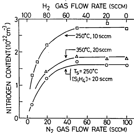
FIGURE 9.2 Nitrogen content of GD a-Si:N:H films.
