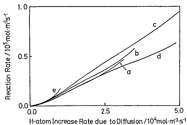
Ffg. 11. Rates of reaction (R5), \text{OH} + \text{H}_2 \rightarrow \text{H} + \text{H}_2\text{O} , as functions of the rate of the increase in hydrogen atoms due to diffusion.
