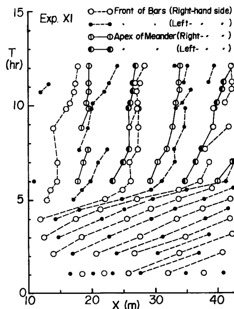
Fig. 2 Migration of fronts of bars and location of meander.
