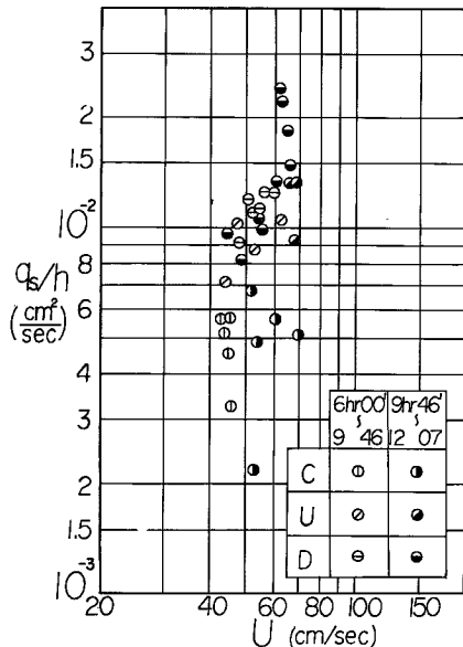
Fig. 19 Relation between bank erosion rate and mean velocity along meandering bend (C: Crossing of meandering channel, U: Upstream part of meandering bend, D: Downstream part of meandering bend).
