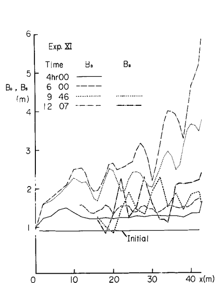
Fig. 14 Variation of channel width ( B_D ) and bed load width ( B_S ).
