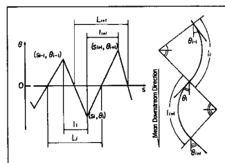
Fig. 11 Schematic sketch of meandering stream.
