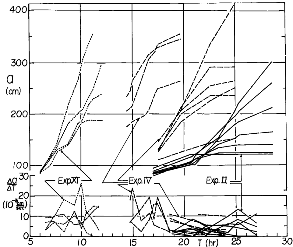
Fig. 3 Variation of amplitude and rate of amplification of meandering channels.
