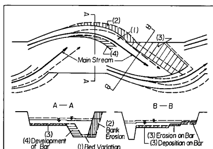
Fig. 12 Schematic sketch of process of meandering channel development.
