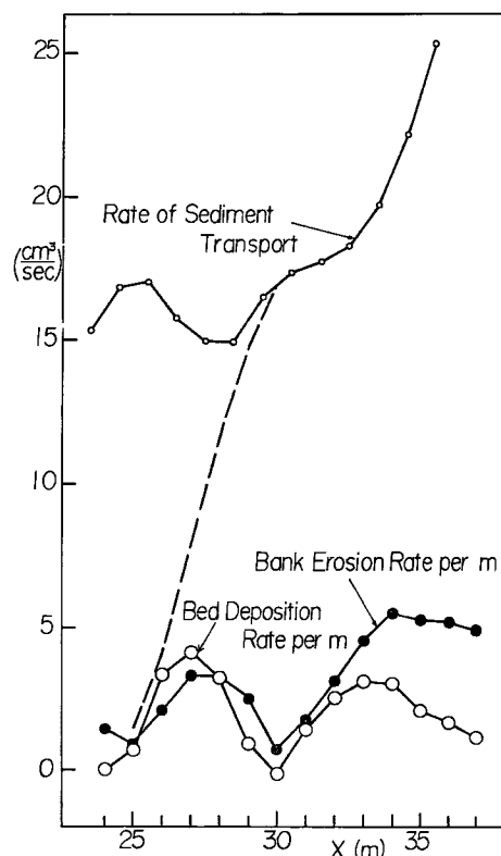
Fig. 20 Comparison among rate of sediment transport, bank erosion rate and bed deposition rate.
