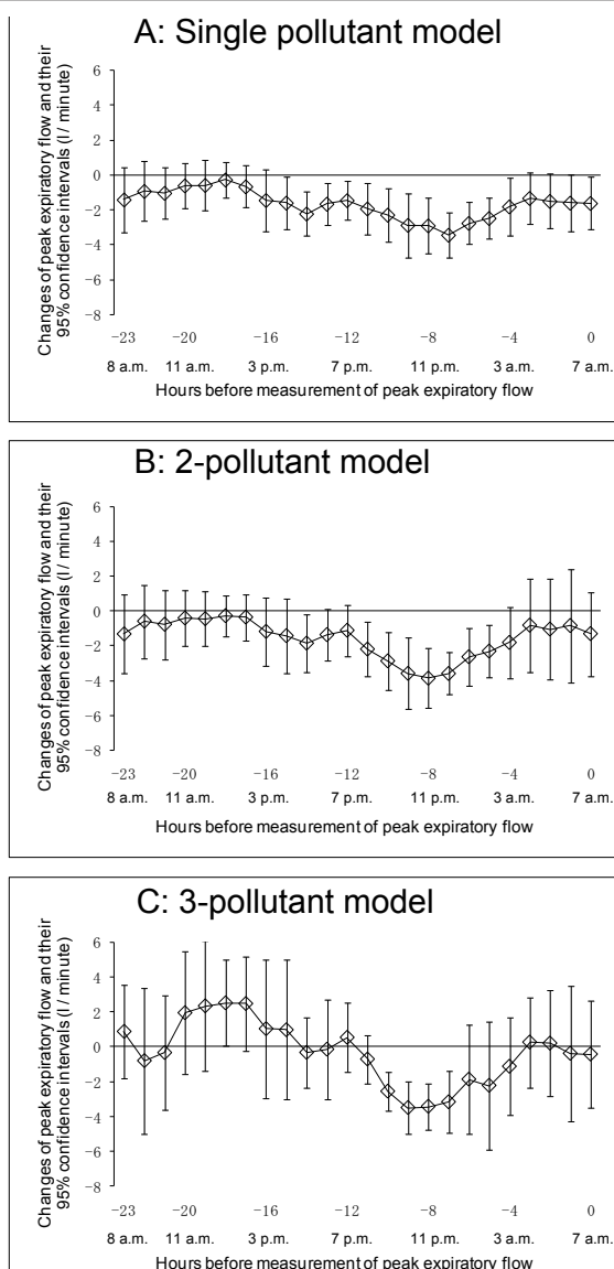
Figure 2 Association between PEF measured in the morning at 7 a.m. and hourly concentration of PM_{2.5} . Lagged-hour exposures of up to 24 hours were examined. The mean differences and 95% confidence intervals in PEF per 10 \mu g/m^3 increases in PM_{2.5} were estimated. A: Single-pollutant model adjusted for age, sex, height, day of the week, temporal trends, and temperature. B: 2-pollutant model adjusted for age, sex, height, day of the week, temporal trends, photochemical oxidants, and temperature. C: 3-pollutant model adjusted for age, sex, height, day of the week, temporal trends, nitrogen dioxide, photochemical oxidants, and temperature.
