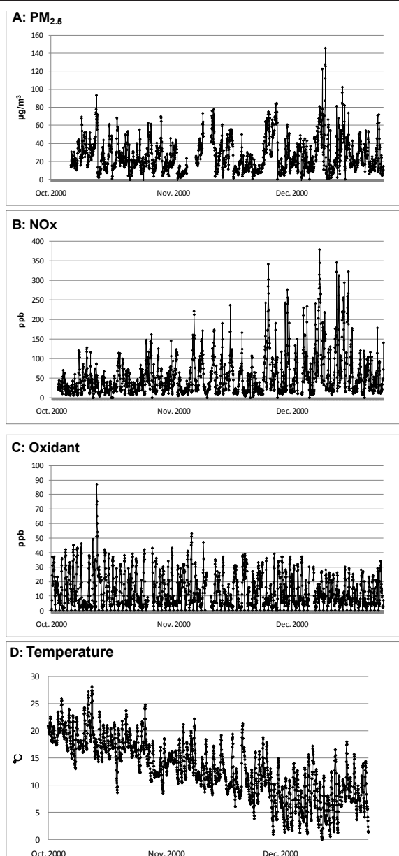
Figure 1 Hourly concentration of air pollutants and hourly temperature from October 1, 2000 through December 24, 2000. A: PM 2.5 B: NOx C: Ox D: Temperature.
