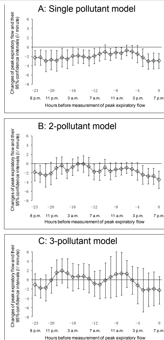
Figure 3 Association between PEF measured in the evening at 7 p.m. and hourly concentration of PM_{2.5} . Lagged-hour exposures of up to 24 hours were examined. Mean differences and 95% confidence intervals in PEF for 10 \mu g/m^3 increases in PM_{2.5} were estimated. A: Single-pollutant model adjusted for age, sex, height, day of the week, temporal trends, and temperature. B: 2-pollutant model adjusted for age, sex, height, day of the week, temporal trends, photochemical oxidants, and temperature. C: 3-pollutant model adjusted for age, sex, height, day of the week, temporal trends, nitrogen dioxide, photochemical oxidants, and temperature.
