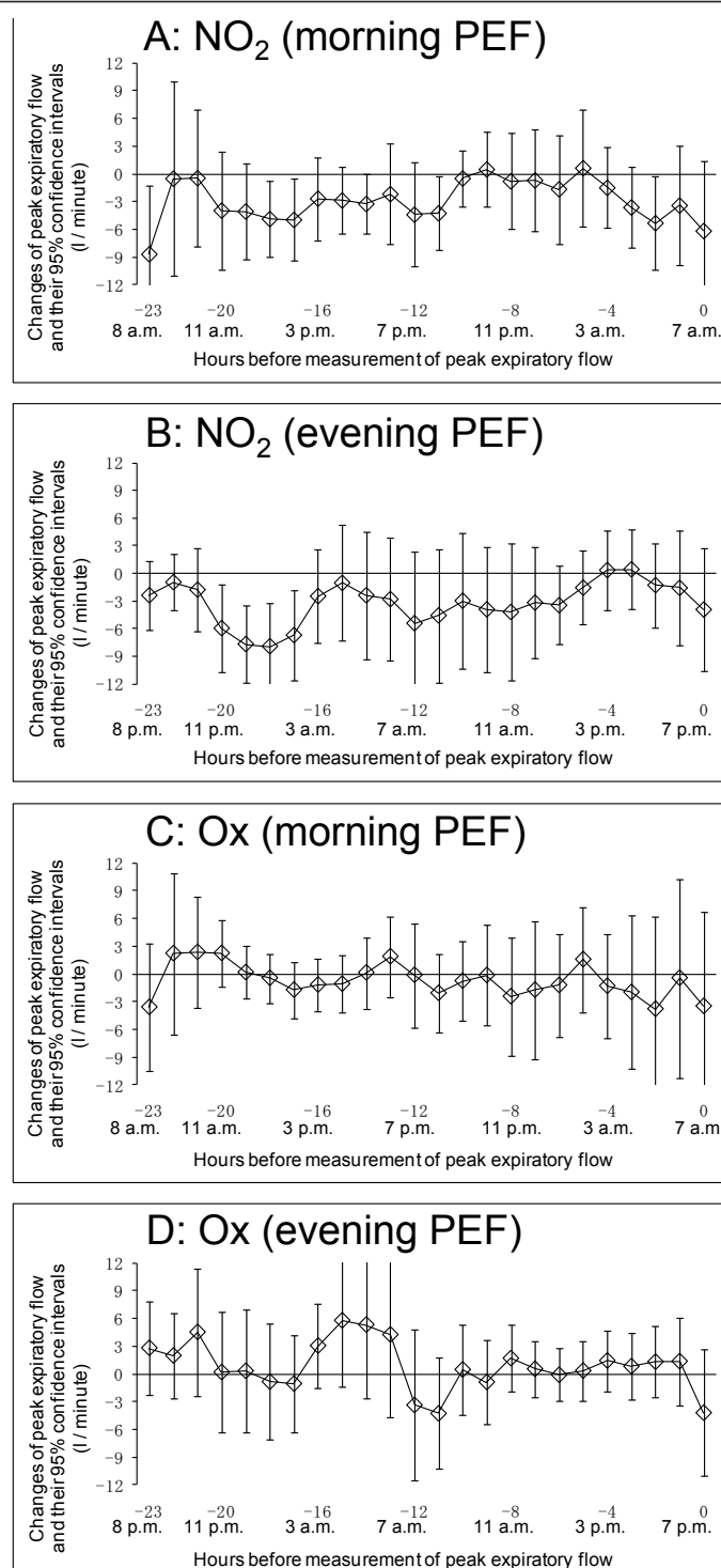
Figure 5 Association between PEF and hourly concentration of other pollutants (NO 2 and Ox) using 3-pollutant model. Lagged-hour exposures of up to 24 hours were examined. Mean differences and 95% confidence intervals in PEF for 10 ppb increases in NO 2 /Ox were estimated using 3-pollutant model adjusted for age, sex, height, day of the week, temporal trends, and temperature. A: Association between PEF measured in the morning at 7 a.m. and hourly concentration of NO 2 . B: Association between PEF measured in the evening at 7 p.m. and hourly concentration of NO 2 . C: Association between PEF measured in the morning at 7 a.m. and hourly concentration of Ox. D: Association between PEF measured in the evening at 7 p.m. and hourly concentration of Ox.
