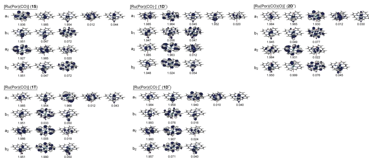
Figure A2. CASSCF-calculated natural orbitals and their occupation numbers of [\text{Ru}(\text{Por})(\text{CO})] and [\text{Ru}(\text{Por})(\text{CO})(\text{O})]^- .
