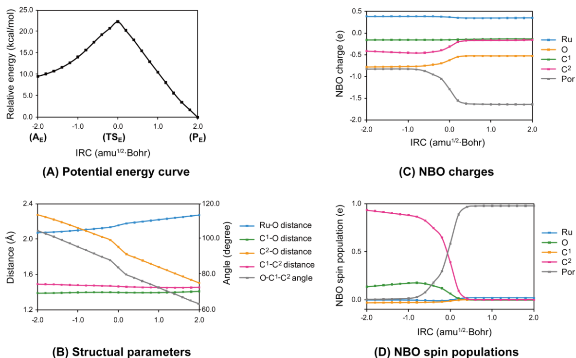
Figure 7. Potential energy curve (A), structural parameters a) (B), NBO charges (C), and NBO spin populations (D) along intrinsic reaction coordinate (IRC) for the ethylene epoxidation. a) see Figure 3 for the C 1 and C 2 atoms.
