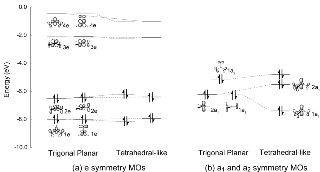
(A) Selected molecular orbitals of \text{Os}(\text{NAr})_3 at tetrahedral-like and trigonal planar geometries
