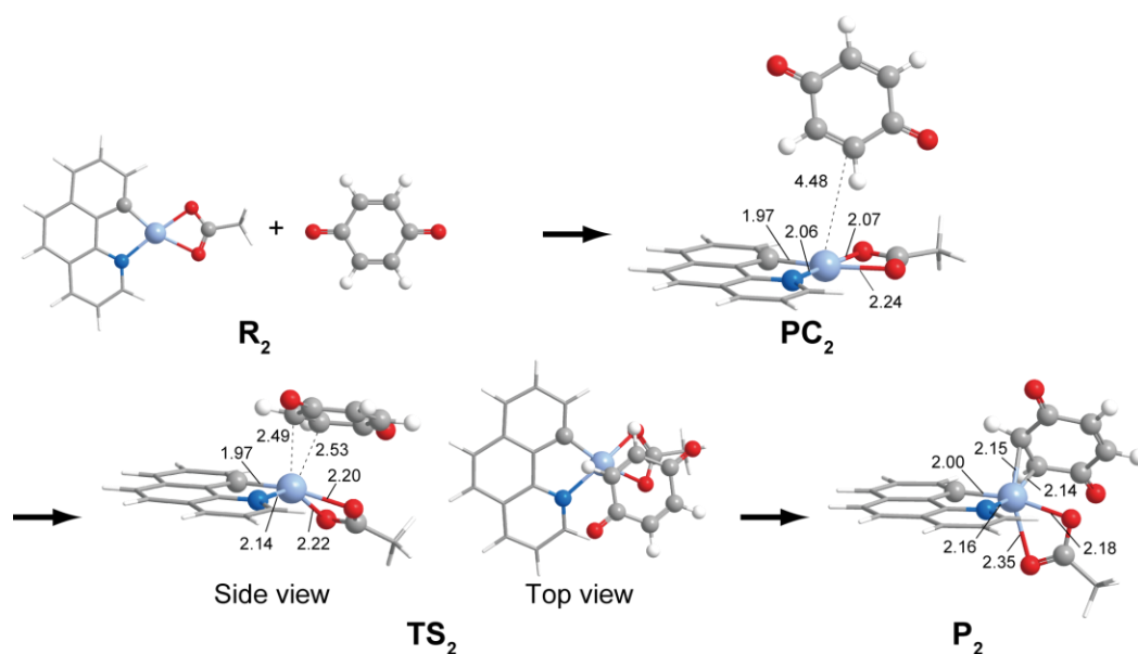
Fig. 4. Geometry changes in the BQ coordination to Pd(Bzq)(OAc). Bond lengths are in Å and bond angle are in degrees.
