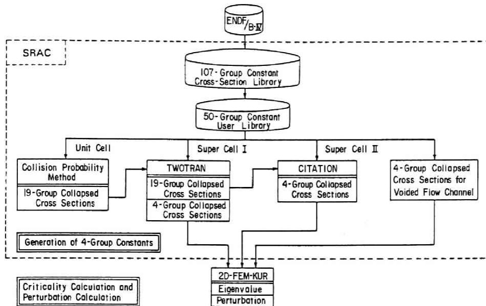
Fig. V-1 Flow Chart for the Calculation
