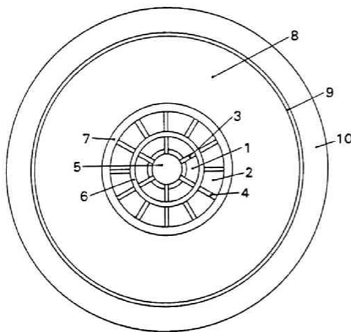
Fig. V-2 Core Configuration Used in the Diffusion Calculation
