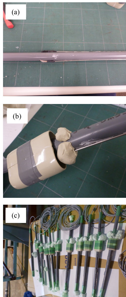
Photo 1 Production processes of a TDR
