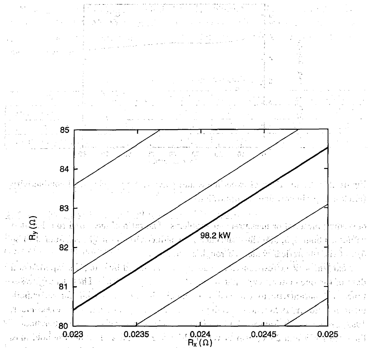
Figure 2.10: Effects of leakage resistances in the x - and y -directions on power output, (difference of lines:1 kW, the bold line:98.2 kW)
