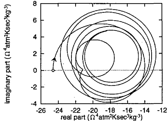
Figure 4.18: Locus of \Delta(j\omega)(\omega \geq 0) of the newly designed generator with ohmic loads when p_{\text{sint}} , T_{\text{sint}} and p_{\text{sext}} are kept constant
