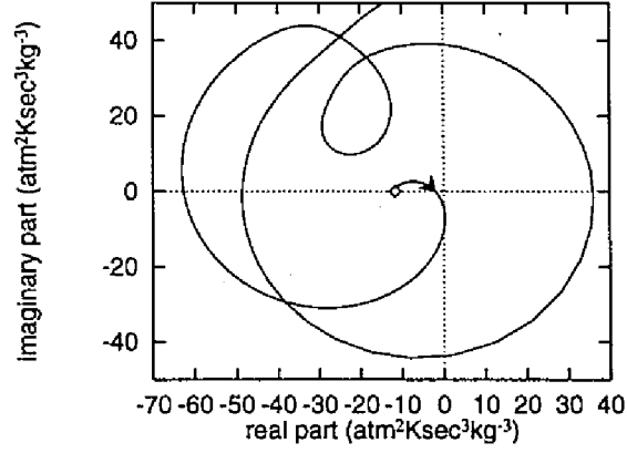
Figure 4.6: Locus of \Delta(j\omega) ( \omega \geq 0 ) under constant current loading condition when T_s , p_s are kept constant at inlet and p_s is kept constant at exit (conventionally designed MHD generator)
