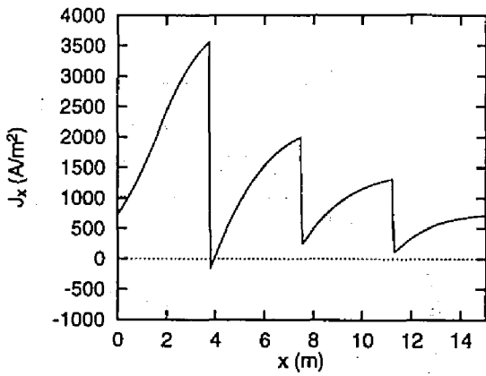
(i) Electric current density in x -direction
