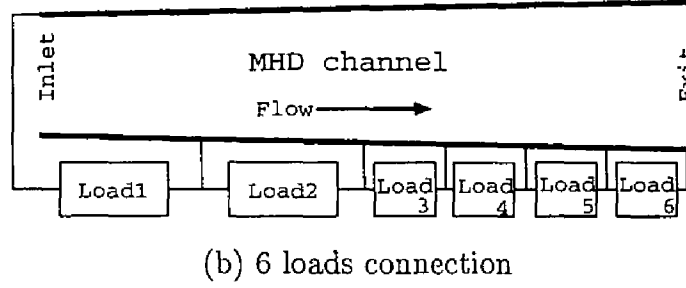
Figure 3.7: Load circuit
