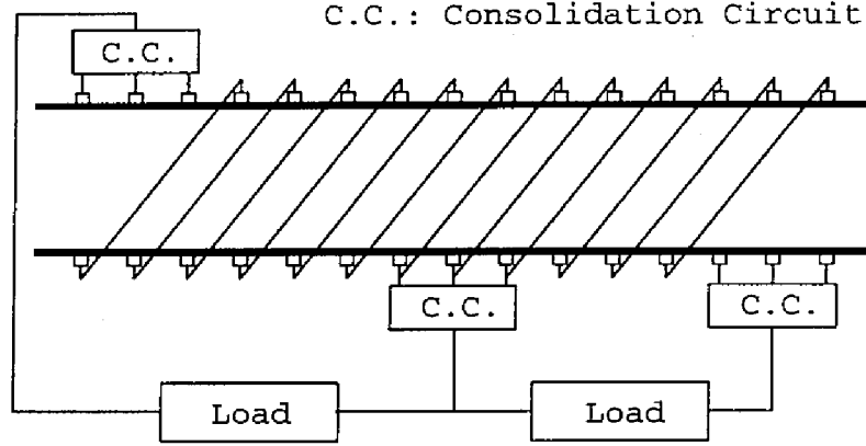
Figure 3.1: Diagonal type MHD generator
