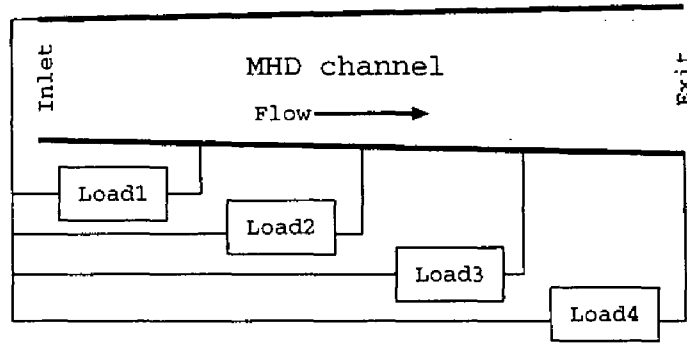
Figure 3.18: MHD generator with feedback loading scheme
