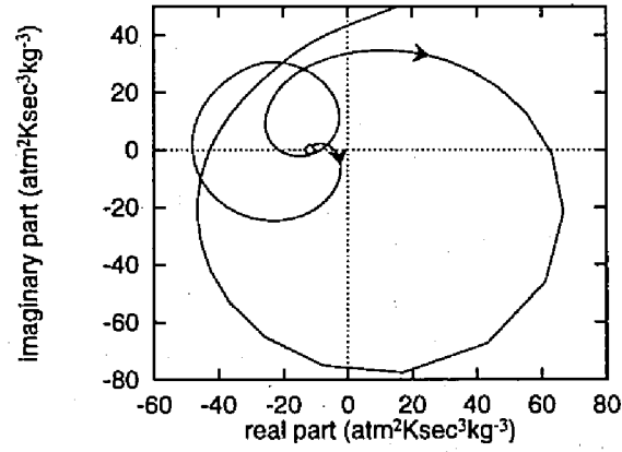
Figure 4.7: Locus of \Delta(j\omega) ( \omega \geq 0 ) under constant current loading condition when T , p are kept constant at inlet and p is kept constant at exit (conventionally designed MHD generator)
