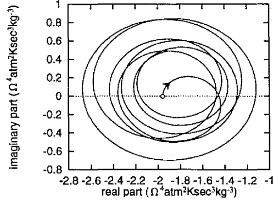
Figure 4.17: Locus of \Delta(j\omega)(\omega \geq 0) of the newly designed generator with constant voltage loads when p_{\text{sint}} , T_{\text{sint}} and p_{\text{sext}} are kept constant
