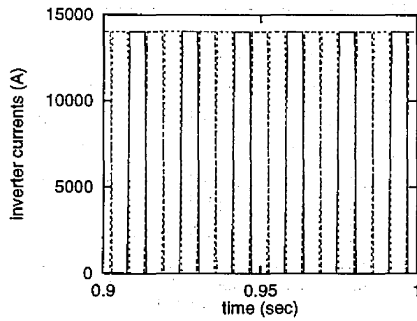
Figure 6.3: Three-phase thyristor currents in inverter #11
