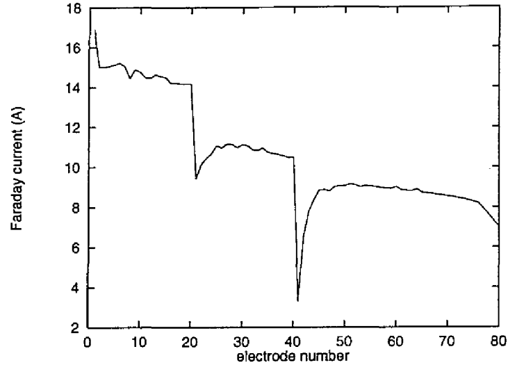
Figure 2.24: Faraday current distribution along channel (power run at November 1994)
