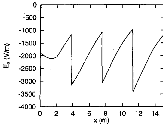
(g) Electric field in x -direction
