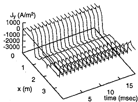
(h) Current density in y -direction
