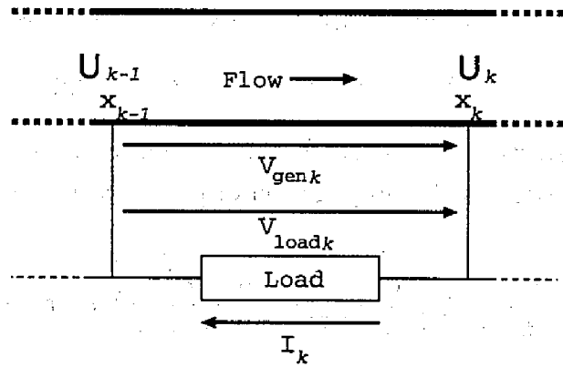
Figure 3.4: k-th loading section
