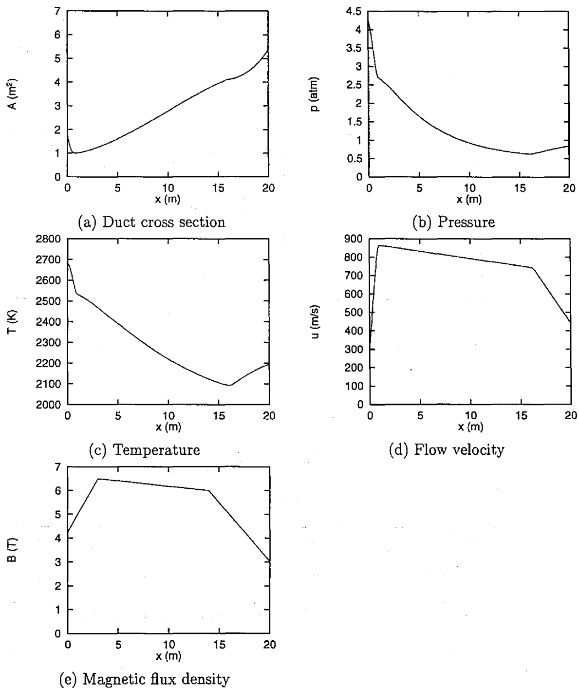
Figure 5.1: Distributions of quantities under design condition
