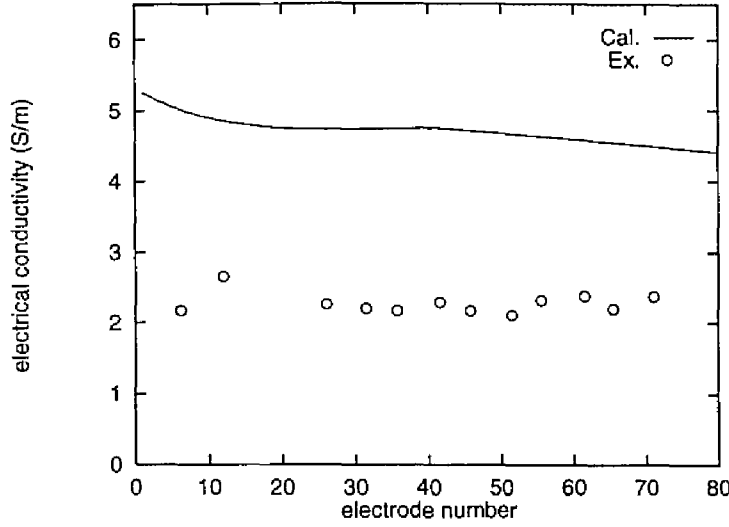
Figure 2.9: Comparison of experiment and computation of electrical conductivity (circles: experiment; line: computation)
