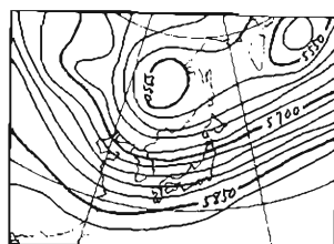
Fig. 10. Same as Fig. 9 but for 12~15 July 1959.
