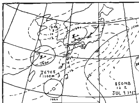
Fig. 26. Same as Fig. 19 but for 21 LST, 9 July 1967.
