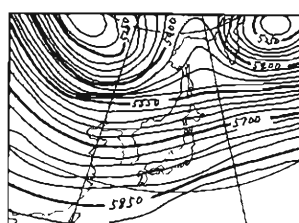
Fig. 11. Same as Fig. 9 but for 1~4 October 1959.
