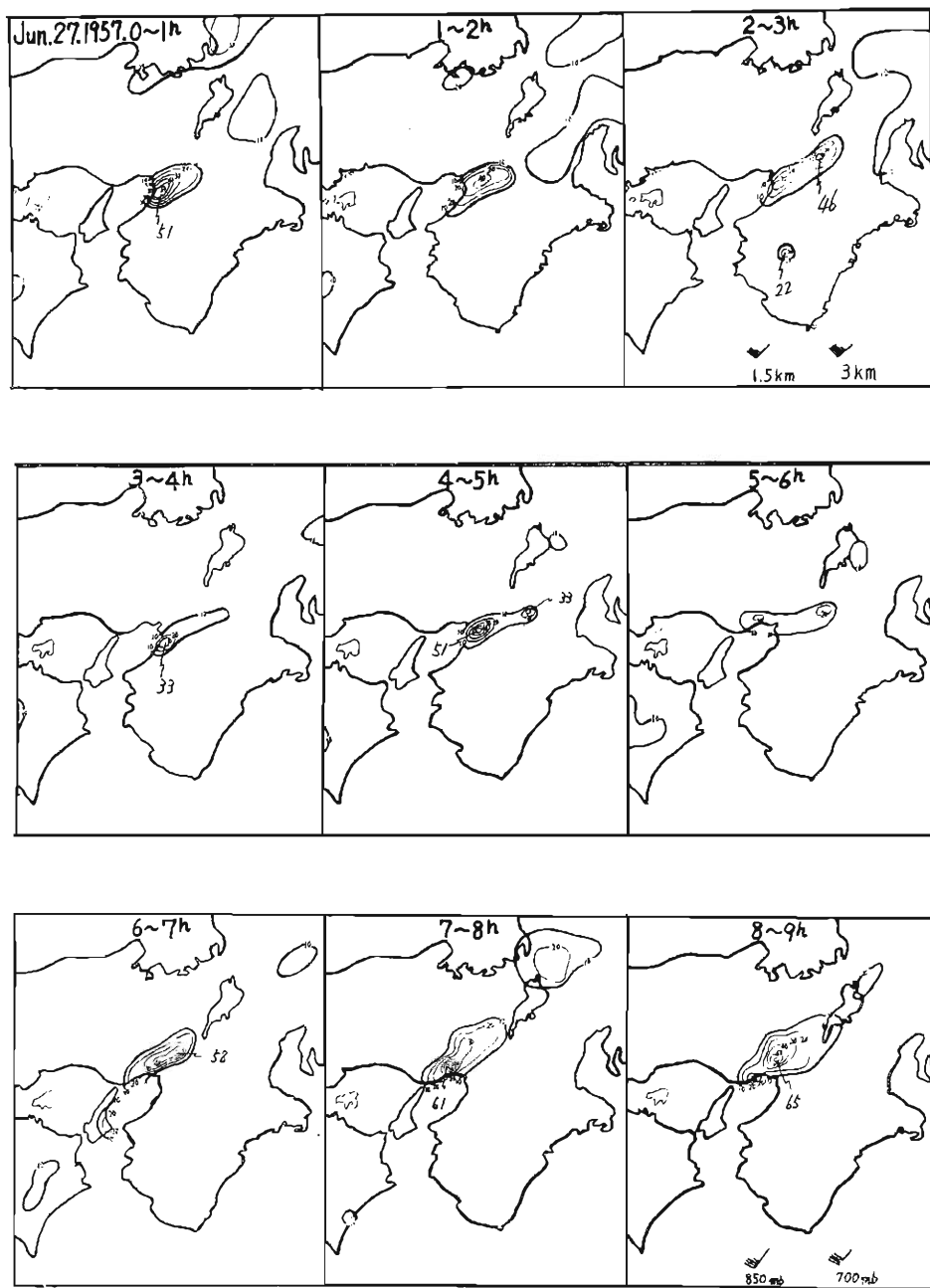
Fig. 20. The hourly rainfall distribution from 01 to 09 LST, 27 June 1957, with the wind (a long barb 10 knots) at the height of 1.5 and 3.0 km at 03 LST and the wind at 850 mb and 700 mb level at 09 and 21 LST.
