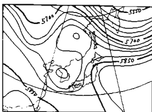
Fig. 9. 4-day mean 500 mb height pattern for 11~14 August 1958.
