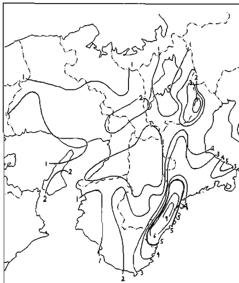
Fig. 5. Total number of days when daily precipitations are 101 mm or more in warm season.
