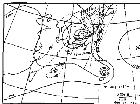
Fig. 21. Same as Fig. 19 but for 21 LST, 29 August 1960.
