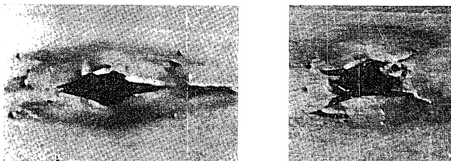
Fig. 4. Pictures showing the broken states of the Wood structure. Left : by static driving; Right : by impact driving
