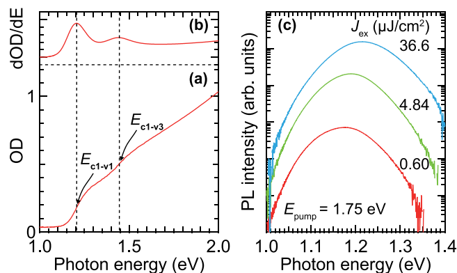
FIG. 2. (a) Absorption spectrum and (b) first-order derivative of the absorption spectrum of CIGS thin films. (c) Dependence of steady-state PL spectra of CIGS thin films on the excitation fluence ( J_{ex} ) with photoexcitation ( E_{pump} ) of 1.75 eV.
