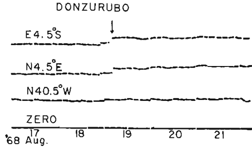
Fig. 4-(c) Strain step records obtained at the Donzurubo Observatory for earthquake No. 14 ( M=5.6 , \Delta=80 km) E04.5^\circ S: -7.4 \times 10^{-8} N04.5^\circ E: -8.1 " N40.5^\circ W: 0 (< 5 \times 10^{-9}) .
