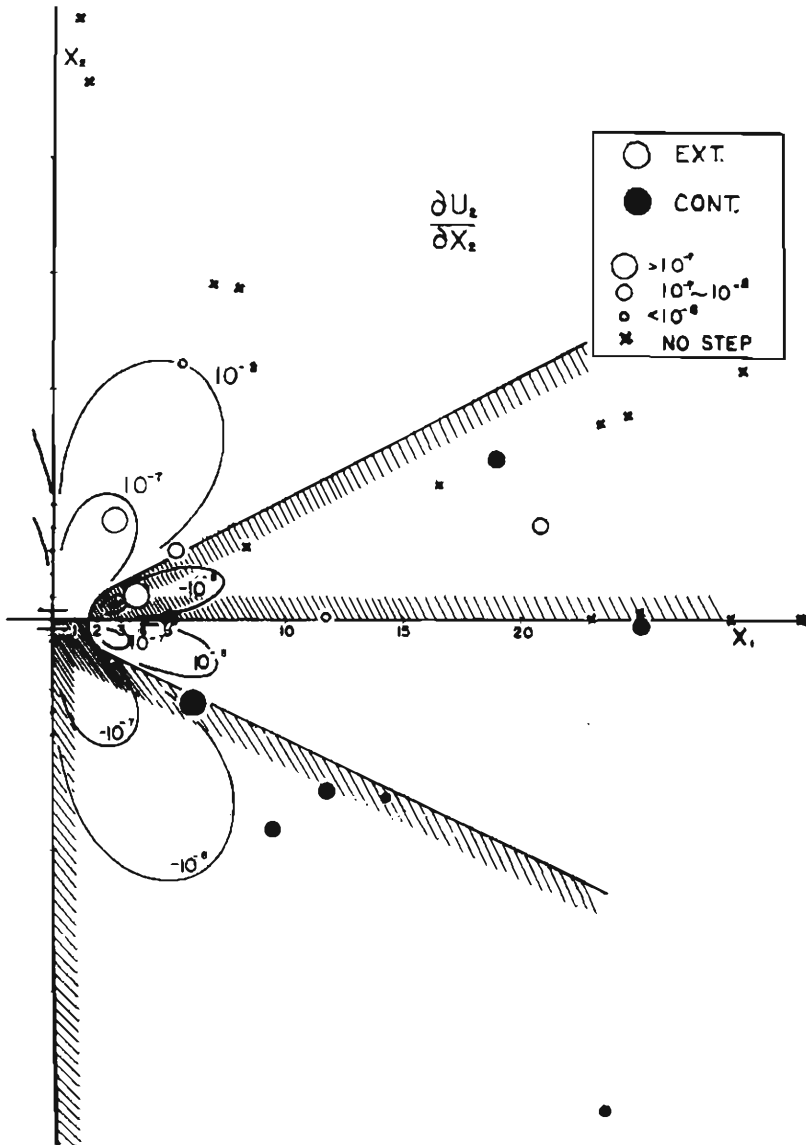
Fig. 7-(b) Observed values of strain step amplitudes and a residual strain field for strike-slip with D=0.5 L and U=1/6 \times 10^{-4} ( X_2 -direction).
