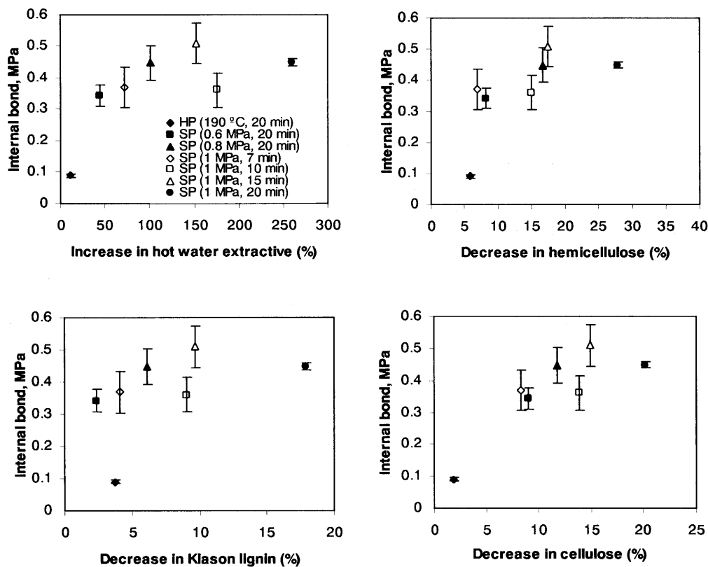
Fig. 1. The effect of chemical changes by steam and heat treatments on internal bond strength of kenaf core binderless boards. The corrected density of binderless boards was 0.5 \text{ g/cm}^3 . HP, hot pressing; SP, steam-injection pressing
