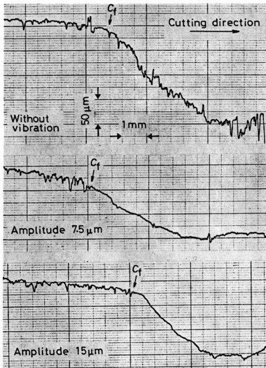
Fig. 5. Profiles of machined surface in inclined cutting. \theta = 1.9^\circ , V_o = 0.69 \text{ mm/s} , 90^\circ - 0^\circ cutting.
