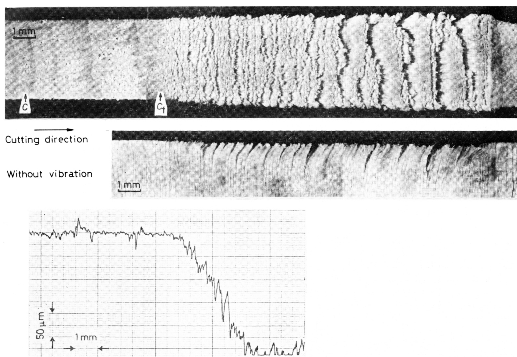
Fig. 6. Machined surface in inclined cutting. \theta=0.7^\circ , V_o=0.69\text{mm/s} , 90^\circ-90^\circ cutting.
