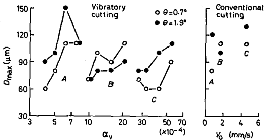
Fig. 8. Relation between maximum deviation D_{max} and cutting speed ratio \alpha_v in 90^\circ-0^\circ cutting. A, V_o=0.69 mm/s; B, V_o=1.72 mm/s; C, V_o=4.60 mm/s.
