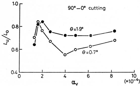
Fig. 4. Relation between contact length ratio L_u/L_o and cutting speed ratio \alpha_v .
