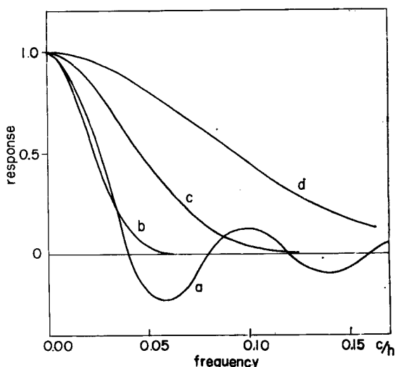
Fig. 1 Frequency response of an equally-weighted running mean and of normal probability curve smoothing function. Curve(a) is response of the 25-hour running mean. Curves (b), (c) and (d) are response of normal curve smoothing functions having 8-, 4- and 2-hour data intervals computed from equation (6), respectively.
