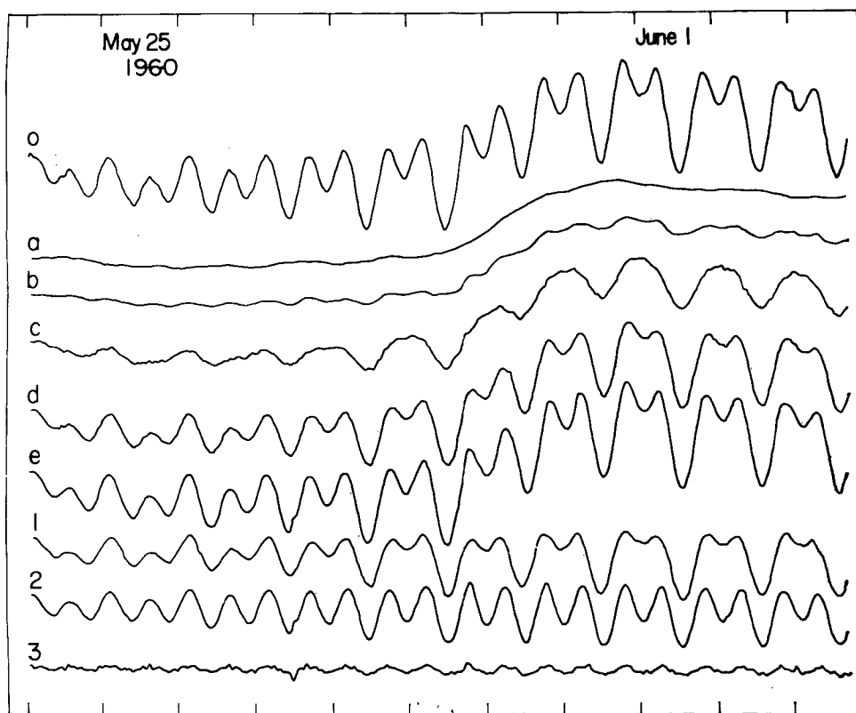
Fig. 4 Examples of filtering of the ground tilt in the N-S direction at Akibasan Observation Station in Wakayama City. Curve (o) is the original ground tilt. Curves (a), (b) and others are filtered time series by filters having response corresponding to curve (a), (b) and others in Fig. 1, Fig. 2 and Fig. 3.
