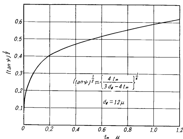
Fig. 20. Variation of (\tan \Psi)^{1/2} with mean cutting depth t_m .
