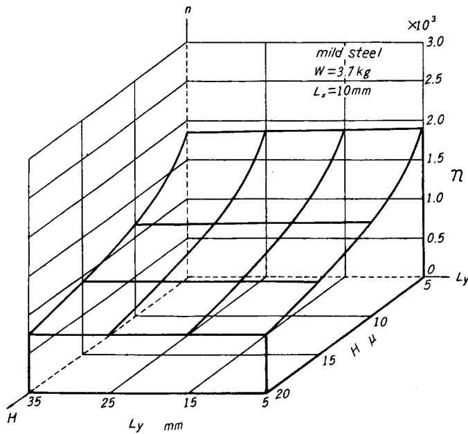
Fig. 15. Variation of number of cutting points n with roughness of stone surface H and stone length L_y obtained under the constant contact load W .
