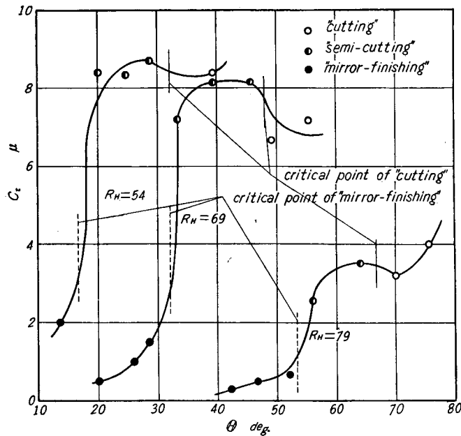
Fig. 16. Variation of cutting depth C_t with cutting direction angle \theta about various bond hardness of stones.
