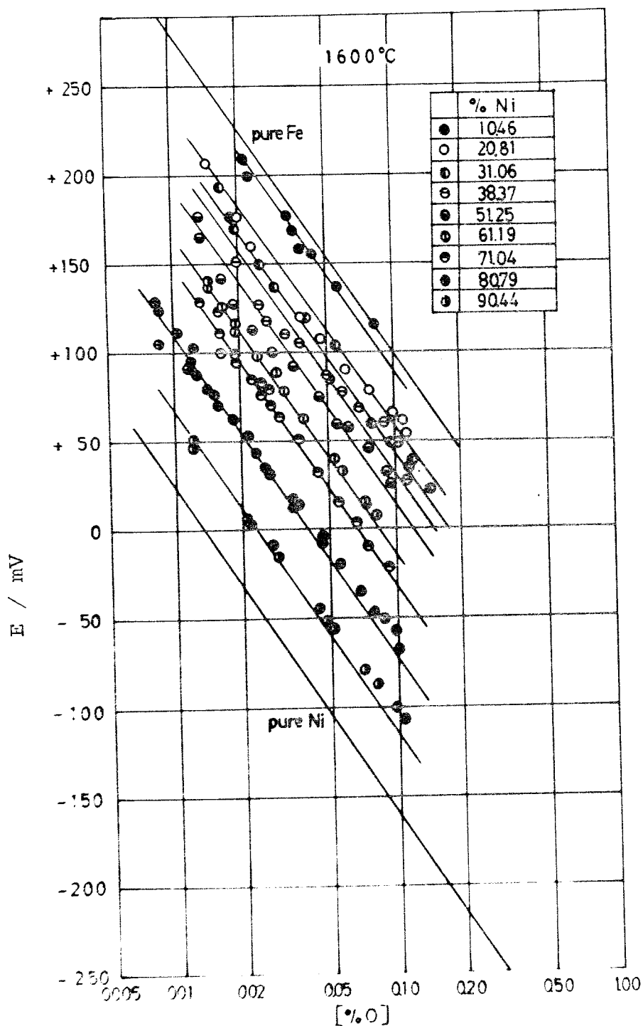
Fig.3.7 Relation between e.m.f. and log[%O] for cell(III).
