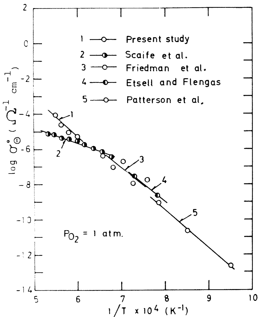
Fig.4.10 The n-type electronic conductivity at P_{O_2} = 1 \text{ atm.} , \sigma^{\circ}_{\Theta} , as a function of reciprocal temperature.
