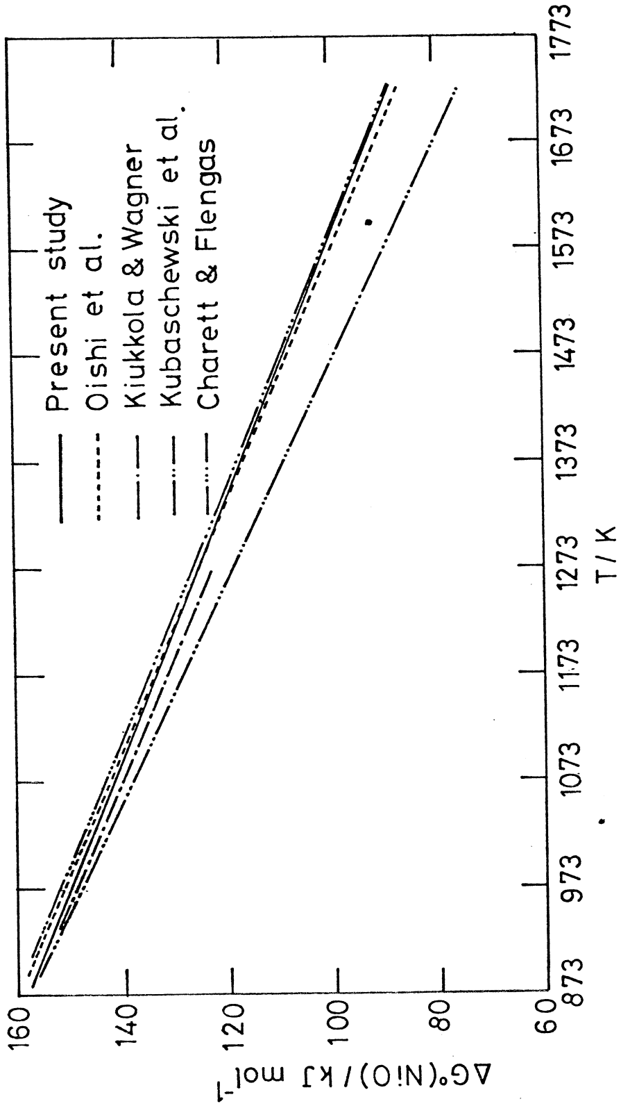
Fig. 2.8 Comparison of the values for standard free nergy of formation of nickel oxide.
