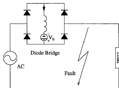
Fig. 1. Main circuit of FCL with diode bridge and DC biased superconducting coil.
