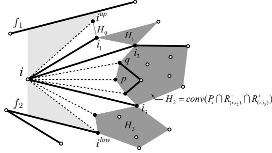
Fig. 2. The part of CSIT around i , where bold edges represent edges of F . Upper and lower light gray regions are empty regions of an upper hull edge (i, i^{up}) and a lower hull edge (i, i^{low}) , respectively. CSIT has edges between i and black vertices.
