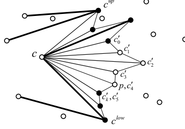
Fig. 4. Existence of an improving flippable edge (c, c'_{j*}) . Bold edges represent the edges of F , and black vertices represent the vertices incident to c in CT^* . In this figure, a quadrilateral cc'_1c'_2c'_3 is convex and (c, c'_2) is improving flippable.
