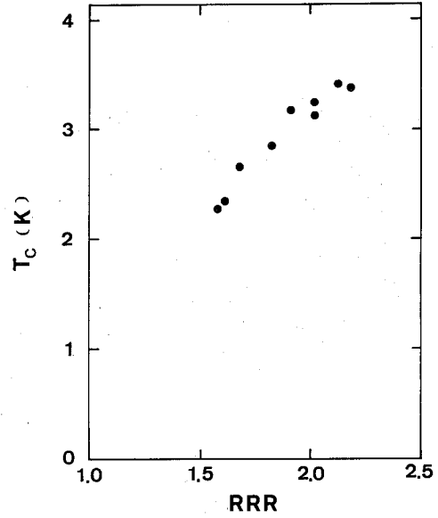
Fig. 4. T_c versus the residual resistance ratio RRR.
