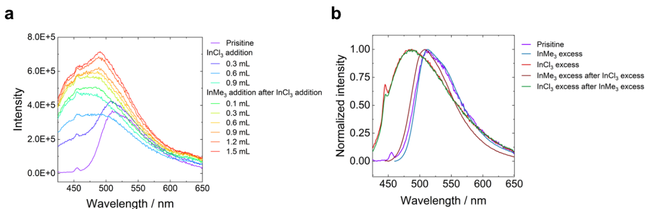
Figure S11. The changes in photoluminescence spectra of a 1.0 \times 10^{-5} \text{ M} solution of PhInMe with (a) stepwise additions and (b) excess additions of \text{InCl}_3 and/or \text{InMe}_3 .
