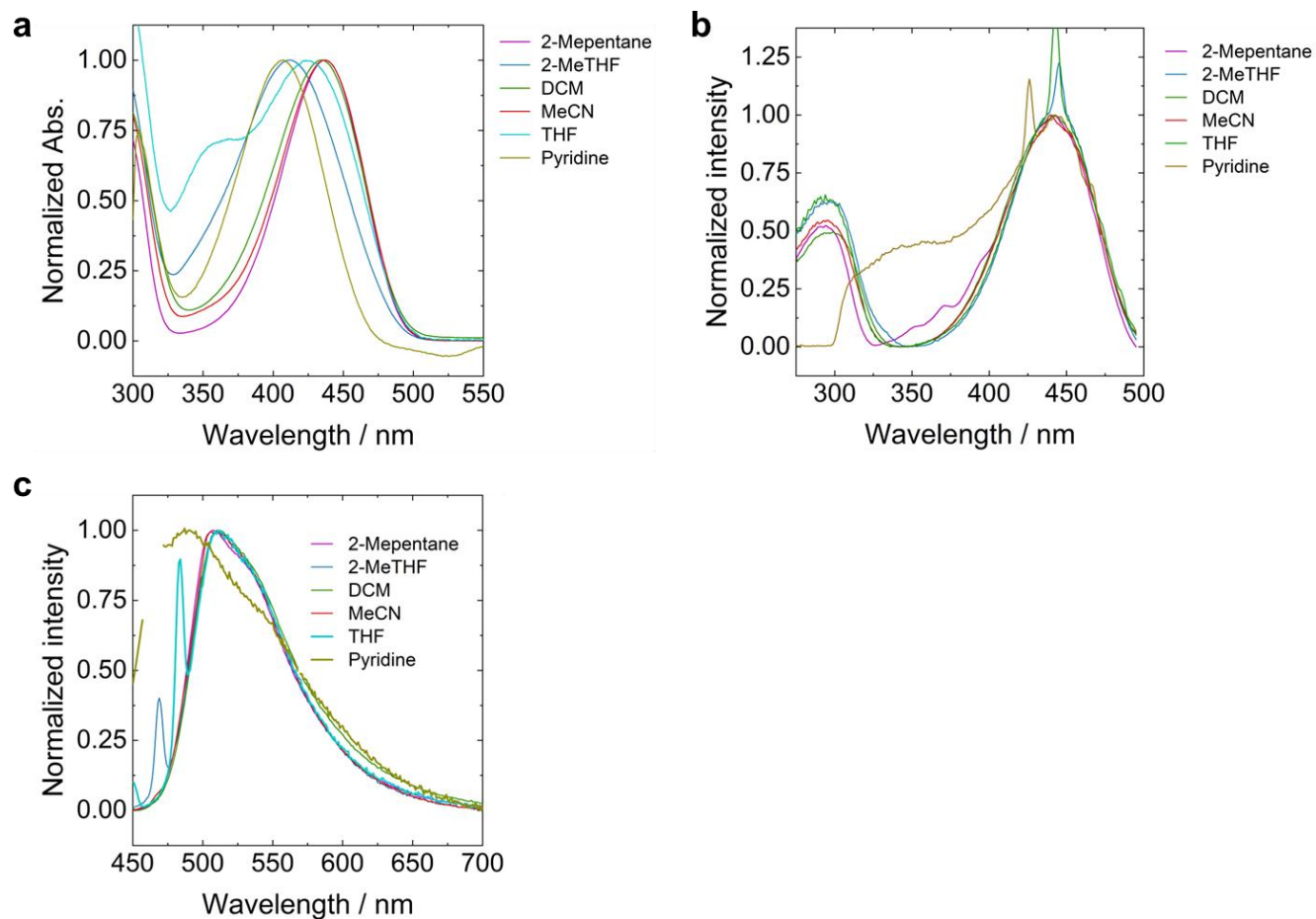
Figure S15. Normalized (a) absorption, (b) excitation, and (c) photoluminescence spectra of PhInMe in various solutions (1.0 × 10 -5 M) at room temperature. Excited at each absorption maximum.
