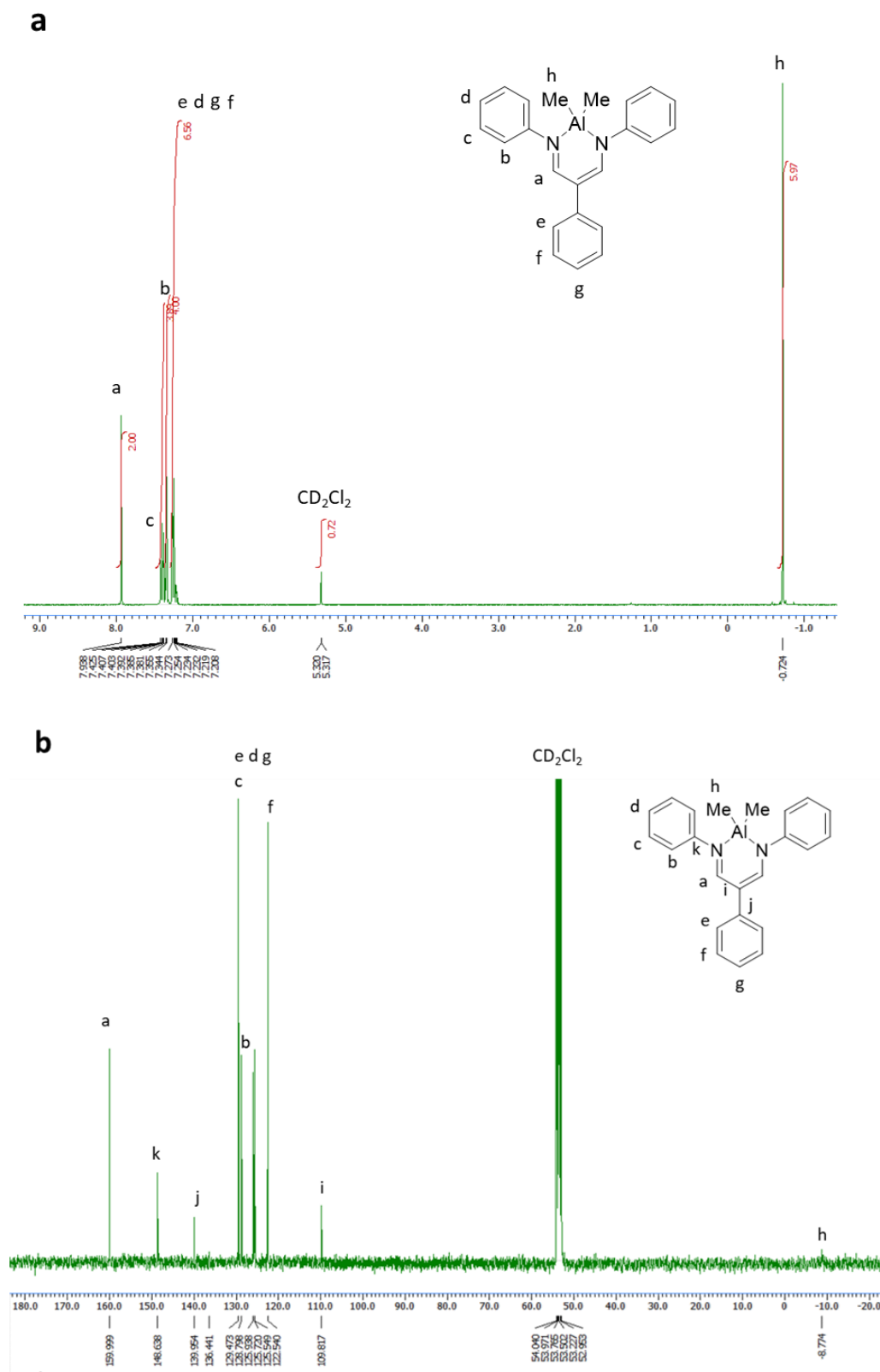
Figure S3. (a) ^1\text{H} and (b) ^{13}\text{C} NMR spectrum of PhAlMe in \text{CD}_2\text{Cl}_2 .
