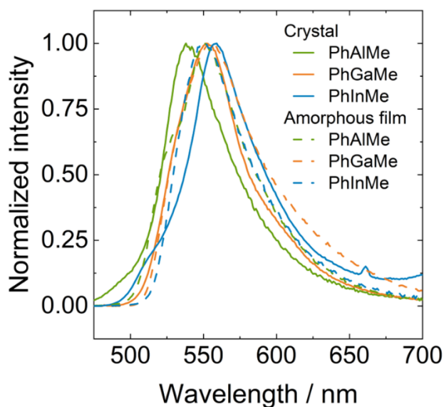
Figure S20. Normalized photoluminescence spectra of the synthesized complexes in their solid states (excited at each absorption maximum of CH 2 Cl 2 solution at room temperature).
