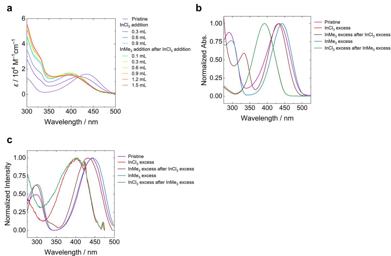
Figure S10. (a) Changes in absorption spectra of a 1.0 \times 10^{-5} \text{ M} solution of PhInMe with the subsequent addition of the saturated \text{InCl}_3 and \text{InMe}_3 solutions in \text{CH}_2\text{Cl}_2 . Changes in (b) absorption and (c) excitation spectra of a 1.0 \times 10^{-5} \text{ M} solution of PhInMe with the additions of \text{InCl}_3 and/or \text{InMe}_3 .
