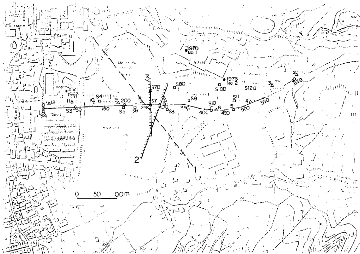
Fig. 5. Measuring line in the present exploration and the positions of the Obaku fault presented by various authors; 1; Mino and Takeuchi 2) , 2; Irikura and Kawana after Kitsunezaki et al. 4) , 3; the present study. No. 1 and 2 denote boreholes in the Obaku Hospital and Pool that in the Uji-City Pool.
