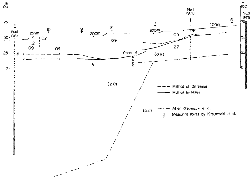
Fig. 12 Comparison between underground structures determined by Kitsunezaki et al. 4) and in the present study.
