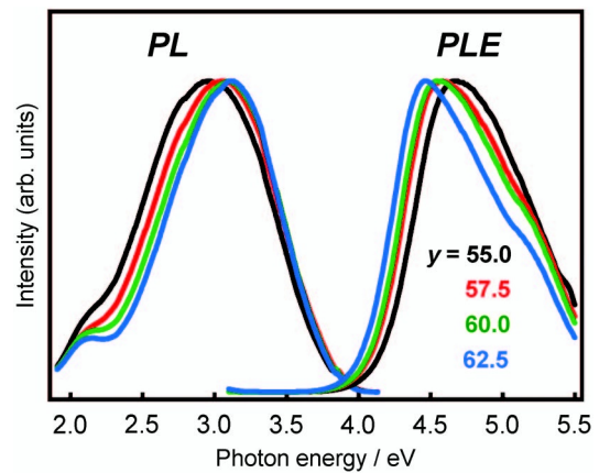
Fig. 2. PL and PLE spectra of 0.5MnO-2.5SnO- y\text{ZnO}-(97.5-y)\text{P}_2\text{O}_5 glasses.
