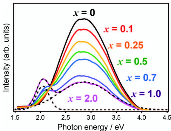
Fig. 1. Correlation between PL intensity excited by 4.88 eV and the amount of Mn in the x\text{MnO}-2.5\text{SnO}-57.5\text{ZnO}-40\text{P}_2\text{O}_5 glasses.
