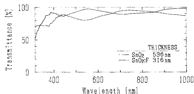
FIG. 3. Optical transmittances of \text{SnO}_2 film and \text{SnO}_2\text{:F} film deposited on borosilicate glass substrate.
