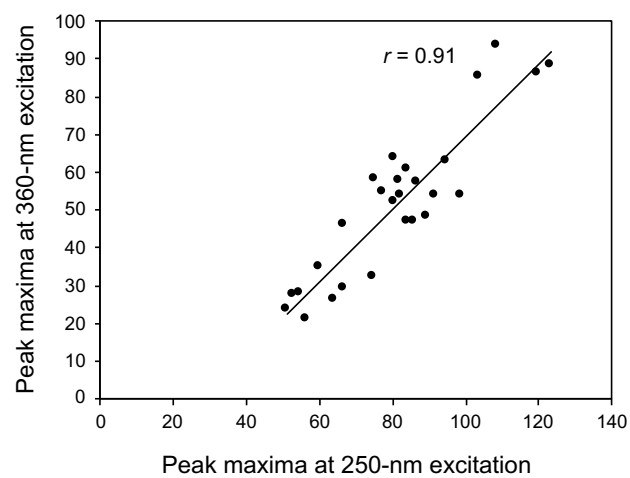
Fig. S2. Relationship between the fluorescence peak maxima at 360 and 250 nm of excitation (28 fruit)
