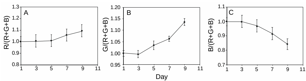
Fig. 6. Relative R (A), G (B), and B (C) ratios of fluorescence color of tomatoes calculated from the fluorescence images: tomatoes were harvested at the red stage and stored at 25°C until day 9, and the colors were averaged for the blossom end without distal area — the error bar represents the S.E. of the same three fruits
