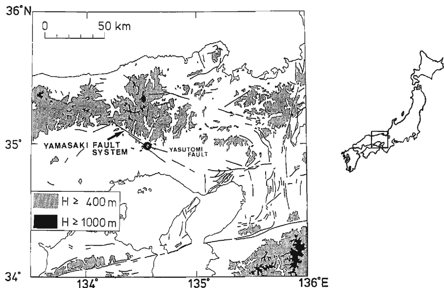
Fig. 1. Map of the northern part of the Kinki District, Southwest Japan. Open circle indicates the Yasutomi-Uzuzuku Baseline Network. Solid lines show main active faults.
