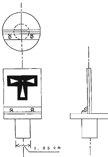
Fig. 4. Sketches showing the design of the target. The target pattern was printed on the film. As the measurements were done at night, it is illuminated with a small lamp from behind.
