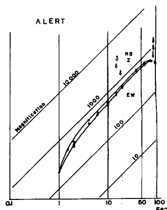
Fig. 2 An example of magnification curve of the Press-Ewing long-period seismograph. The white and black arrows show the periods of the pendulum and galvanometer, respectively.
