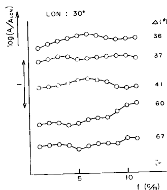
Fig. 11 Amplitude ratio of each component wave at various stations to London. The Mexico earthquake, May 11, 1962 (No. 22, Table 1).
