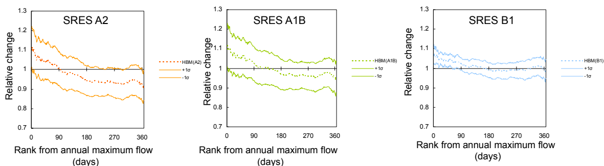
Fig. 9 Change of flow duration curve at Inuyama in the Kiso river basin between present and future climate condition calculated by the Hvdro-BEAM.
