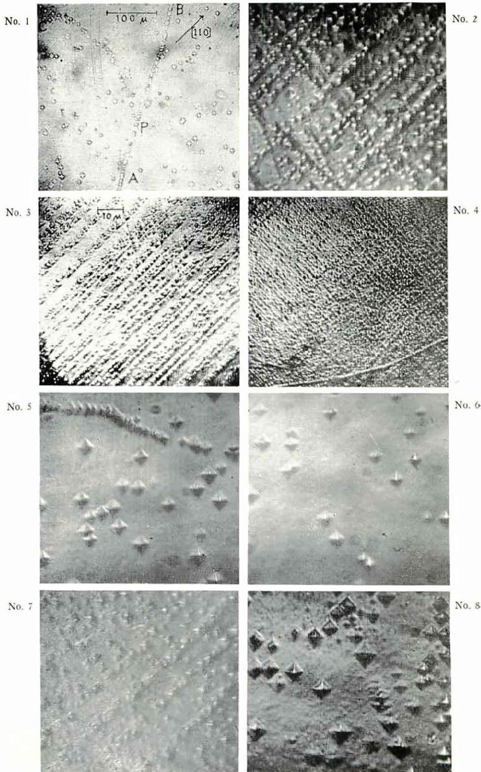
Microphotograph of etch pattern of LiF No. 1: The virgin specimen annealed at 692°C ( \times 150 ), No. 2~4: The specimens compressed at 7500 kg/cm 2 ( \times 800 ), No. 5~6: The specimens compressed at 1620 kg/cm 2 ( \times 800 ), No. 7: The specimen compressed at the hydrostatic pressure of 1000 kg/cm 2 and the uniaxial pressure of 1400 kg/cm 2 ( \times 800 ), No. 8: The specimen cleaved from the optical window for gaseous pressure up to 4000 kg/cm 2 ( \times 800 )
