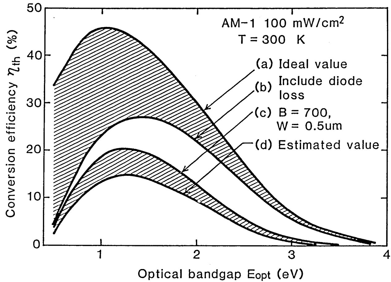
Fig. 5-7 Calculated conversion efficiency as a function of optical bandgap in the case of single bandgap solar cells.
