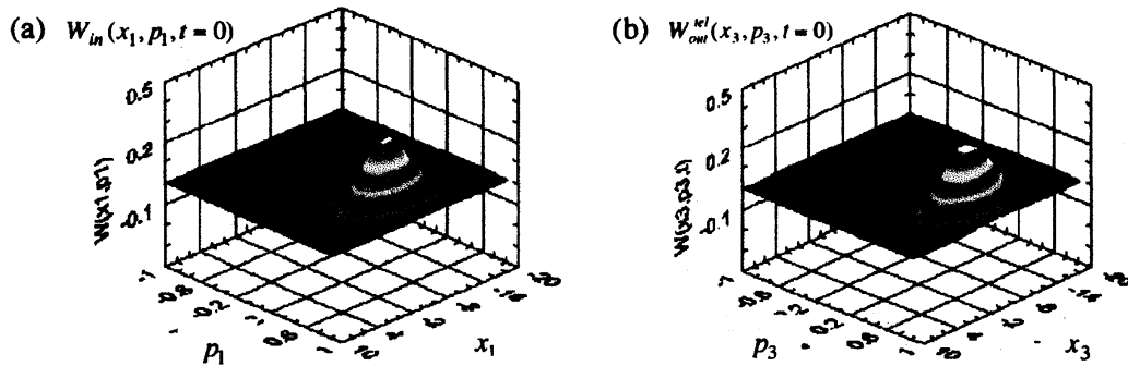
Fig. 8 (a) The Wigner distribution W_{in}(x_1, p_1, t=0) of the one-mode input state |\psi_1(t=0)\rangle = |\phi_1^+(t=0)\rangle . The parameters of |\phi_1^+(t=0)\rangle are the same as those of Fig. 1. (b) The Wigner distribution W_{out}^{tel}(x_3, p_3, t=0) of the output state |\psi_3^{tel}(t=0)\rangle = \hat{U}(a=2, b=1)|\psi_3(t=0)\rangle for the one-mode input state |\psi_1(t=0)\rangle = |\phi_1^+(t=0)\rangle . The parameters are taken as \sigma_{12} = \sigma_{23} = 1.365 , \sigma_{12r} = \sigma_{23r} = 10^3 , a = 2 , b = 1 ( k_1 = 1, k_2 = 0 ). The fidelity is F(t=0) = 0.964 . The units are atomic units.
