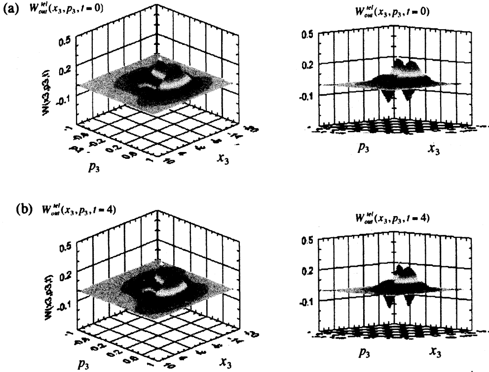
Fig. 4 (a) The Wigner distribution W_{out}^{tel}(x_3, p_3, t=0) of the output state |\psi_3^{tel}(t=0)\rangle = \hat{U}(a=2, b=0.1)|\psi_3(t=0)\rangle for \sigma_{12} = \sigma_{23} = 1.87 . The fidelity is F(t=0)=0.793 . (b) The Wigner distribution W_{out}^{tel}(x_3, p_3, t=4) of the output state |\psi_3^{tel}(t=4)\rangle = U(a=2, b=0.1)|\psi_3(t=4)\rangle for \sigma_{12} = \sigma_{23} = 1.87 . The fidelity is F(t=4)=0.737 . Other parameters are the same as those of Fig. 3. The units are atomic units.
