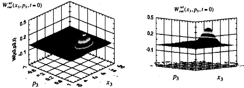
Fig. 7 The Wigner distribution W_{out}^{tel}(x_3, p_3, t=0) of the output state |\psi_3^{tel}(t=0)\rangle = \hat{U}(a=2, b=1)|\psi_3(t=0)\rangle . The parameters are taken as \sigma_{12} = \sigma_{23} = 1.365 , \sigma_{12r} = \sigma_{23r} = 10^3 , a = 2 and b = 1 ( k_1 = 1, k_2 = 0 ). The fidelity is F(t=0) \approx 0.5005 . The input state |\psi_1\rangle is the two-mode state of Eq. (2.1). The parameters of |\psi_1\rangle are the same as those of Fig. 1. The units are atomic units.
