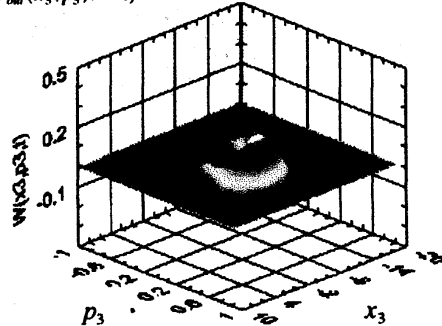
Fig. 6 (a) The Wigner distribution W_{out}^{tel}(x_3, p_3, t=0) of the output state |\psi_3^{tel}(t=0)\rangle = U(a=2, b=0.1)|\psi_3(t=0)\rangle for (\sigma_{12}, \sigma_{23}) = (2.01, 2.03) . The fidelity is F(t=0) = 0.621 . (b) The Wigner distribution W_{out}^{tel}(x_3, p_3, t=4) of |\psi_3^{tel}(t=4)\rangle = U(a=2, b=0.1)|\psi_3(t=4)\rangle for (\sigma_{12}, \sigma_{23}) = (2.01, 2.03) . The fidelity is F(t=4) = 0.567 . The parameters \sigma_{12r} and \sigma_{23r} are taken as \sigma_{12r} = \sigma_{23r} = 20 . Other parameters are the same as those of Fig. 3. The units are atomic units.
