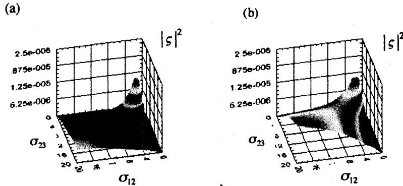
Fig. 2 The behavior of the generating probability |\zeta|^2 for the parameters \sigma_{12} and \sigma_{23} . (a) shows the case of b=0 ( k_1=k_2=0 ). The position of the maximum is \sigma_{12}=\sigma_{23}=1.65 . (b) shows the case of b=0.1 ( k_1=0.1 , k_2=0 ). The position of the maximum is \sigma_{12}=\sigma_{23}=1.87 . The other parameters are taken as \sigma_{12r}=\sigma_{23r}=10^3 , K^\pm=\pm 0.5 , x_0^+=-5 , x_0^-=-7 , k_{12}=k_{23}=0 and a=2 . The units are atomic units.
