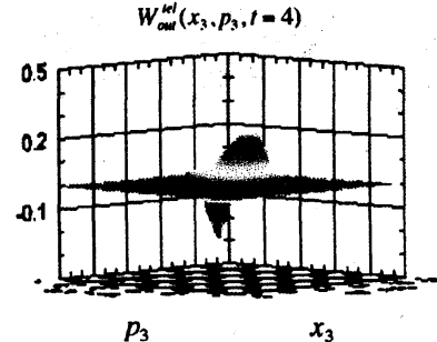
Fig. 6 (a) The Wigner distribution W_{out}^{tel}(x_3, p_3, t=0) of the output state |\psi_3^{tel}(t=0)\rangle = U(a=2, b=0.1)|\psi_3(t=0)\rangle for (\sigma_{12}, \sigma_{23}) = (2.01, 2.03) . The fidelity is F(t=0) = 0.621 . (b) The Wigner distribution W_{out}^{tel}(x_3, p_3, t=4) of |\psi_3^{tel}(t=4)\rangle = U(a=2, b=0.1)|\psi_3(t=4)\rangle for (\sigma_{12}, \sigma_{23}) = (2.01, 2.03) . The fidelity is F(t=4) = 0.567 . The parameters \sigma_{12r} and \sigma_{23r} are taken as \sigma_{12r} = \sigma_{23r} = 20 . Other parameters are the same as those of Fig. 3. The units are atomic units.
