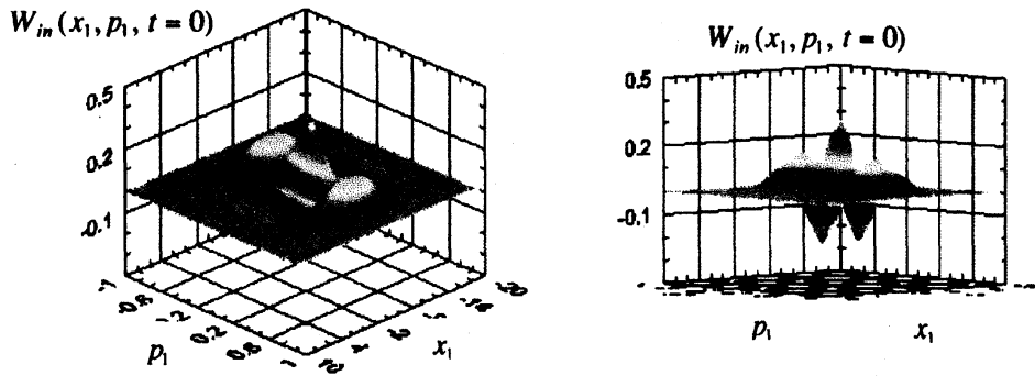
Fig.1 The Wigner distribution W_{in}(x_1, p_1, t=0) of the input state |\psi_1(t=0)\rangle of Eq. (2.1). The parameters of the input state are taken as \sigma_1=5 , K^\pm=\pm 0.5 , x_0^+=-5 , x_0^-=-7 and m=1 . The units are atomic units.
