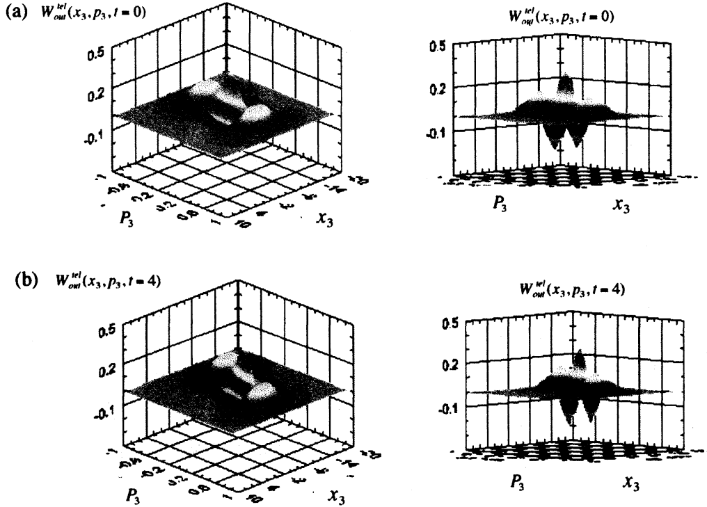
Fig. 3 (a) The Wigner distribution W_{out}^{tel}(x_3, p_3, t=0) of the output state |\psi_3^{tel}(t=0)\rangle = \hat{U}(a=2, b=0.1)|\psi_3(t=0)\rangle . The fidelity is F(t=0) = 0.999 . (b) The Wigner distribution W_{out}^{tel}(x_3, p_3, t=4) of the output state |\psi_3^{tel}(t=4)\rangle = \hat{U}(a=2, b=0.1)|\psi_3(t=4)\rangle . The Fidelity is F(t=4) = 0.885 . The results of the measurement by Alice are assumed to be a=2, b=0.1 ( k_1=0.1, k_2=0 ). The parameters of |\chi_{a,b}\rangle and |\psi_{23}\rangle are k_{23}=k_{23r}=0, \sigma_{12r}=\sigma_{23r}=10^3 and \sigma_{12}=\sigma_{23}=10^{-3} . The units are atomic units.
