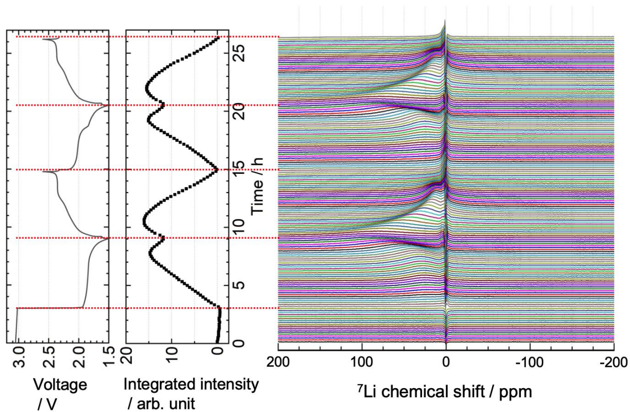
Fig. 2. Time evolution of operando {}^7\text{Li} NMR spectra of the \text{Li}//\text{a-VS}_4 cell, along with the discharge-charge profile and integrated intensity plot of the \text{a-Li}_x\text{VS}_4 signal. The cell was cycled at a current rate of 0.1 C in the voltage window of 1.5–2.6 V. The red dotted lines indicate the start of the discharge or charge process.
