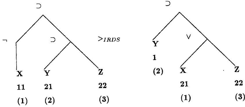
Figure 1: \neg X \supset (Y \supset Z) >_{IRDS} Y \supset (X \vee Z) .
