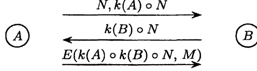
Fig. 2. Diffie-Hellman key exchange algorithm
