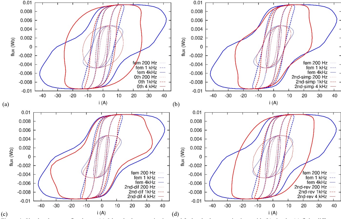
Figure 4: Simulated current-flux loops: (a) 0th order homogenization, and 2nd order homogenizations with (b) simple, (c) finite difference, and (d) reversible approximations.
