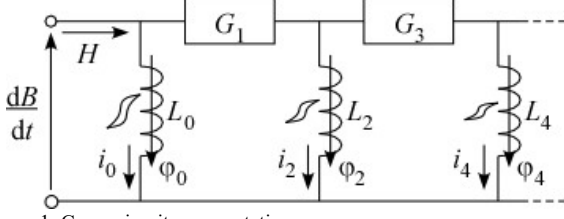
Figure 1: Cauer circuit representation
