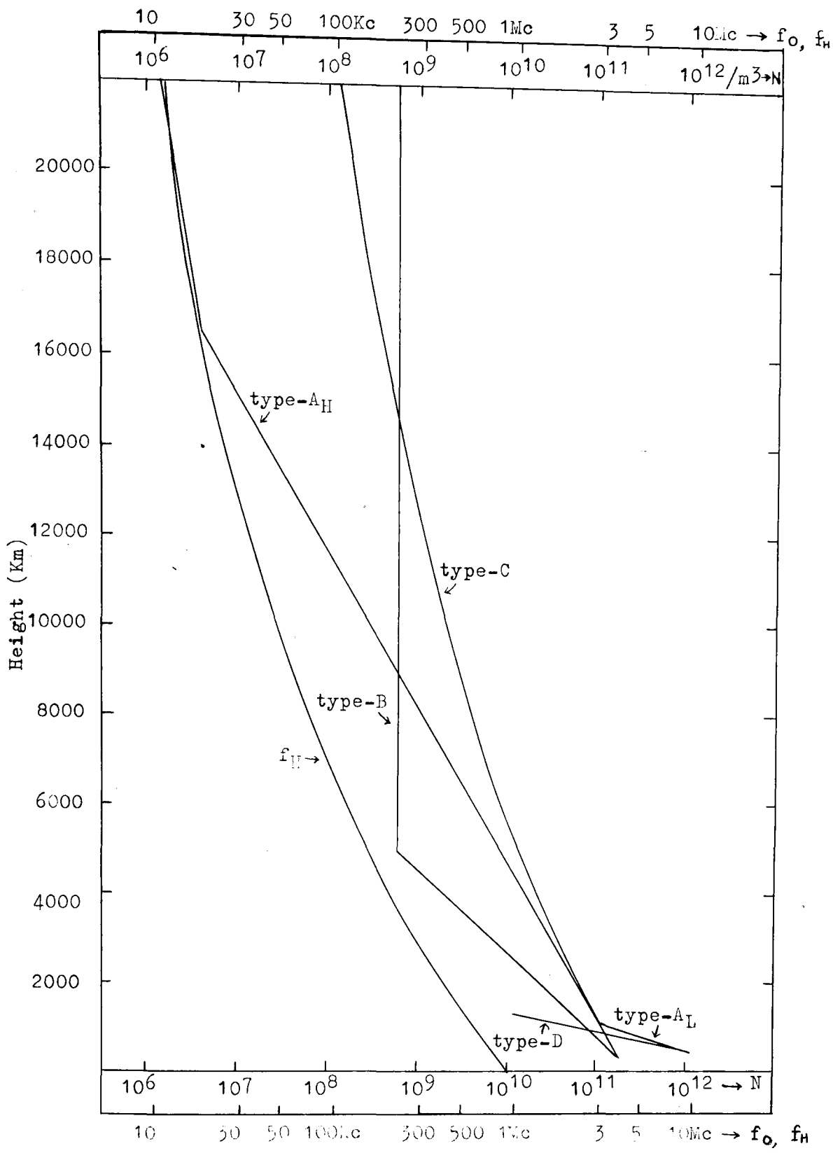
Fig. 1.15 Gyro-frequency and assumed electron density (per m^3 ) against height (km).
