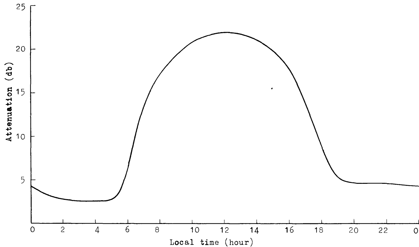
Fig. 1.23 Diurnal variation of the attenuation in the ionosphere for f=3\text{Kc/s} .
