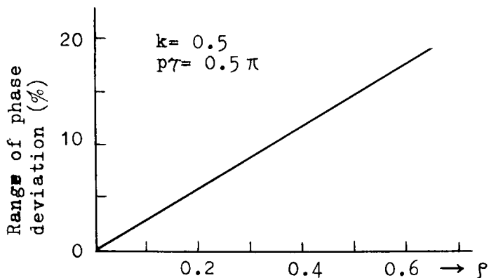
Fig. 3.32 Range of phase deviation as a function of the intermixing ratio \rho .
