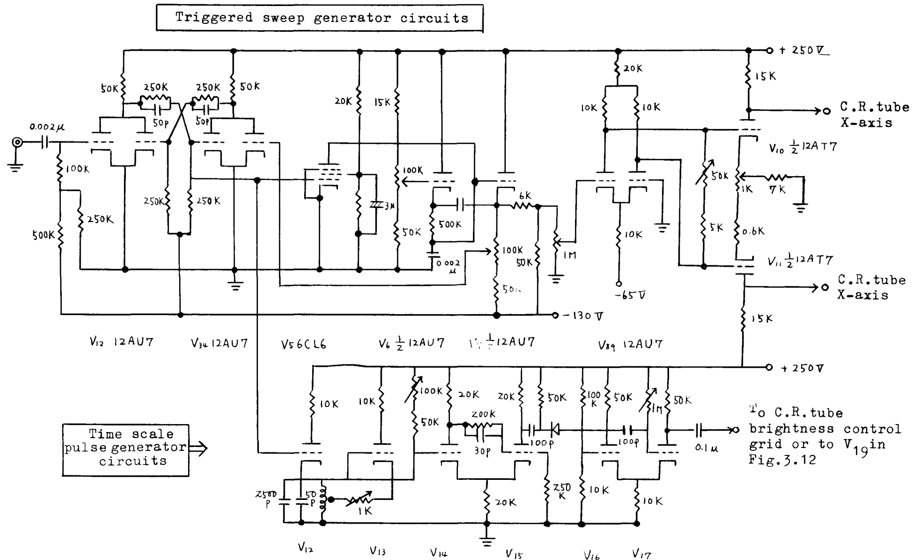
Fig. 3.13 Triggered sweep generator and time scale pulse generator.
