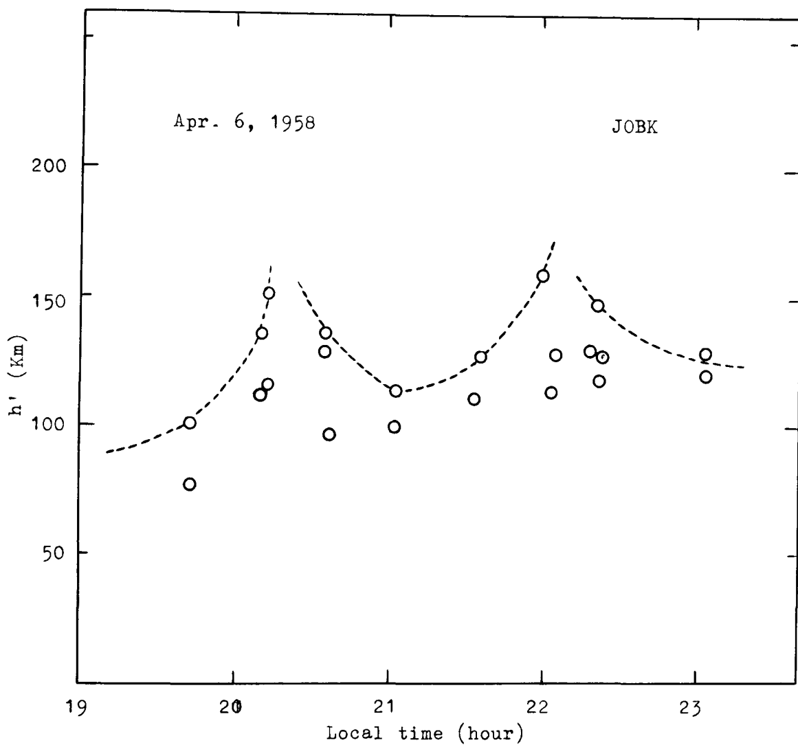
Fig. 3.17 Apparent height h' observed by the direct method. The envelope (dotted line) implies the variation of plausible h' .
