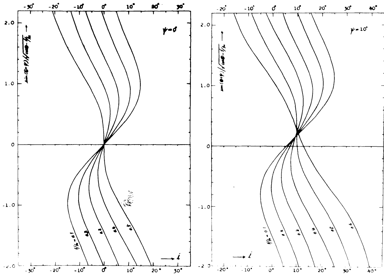
Fig.1.13(a),(b) \sin(\Theta - \psi) / \sqrt{\cos \Theta - f/f_H} against i for \psi = 0^\circ, 10^\circ .
