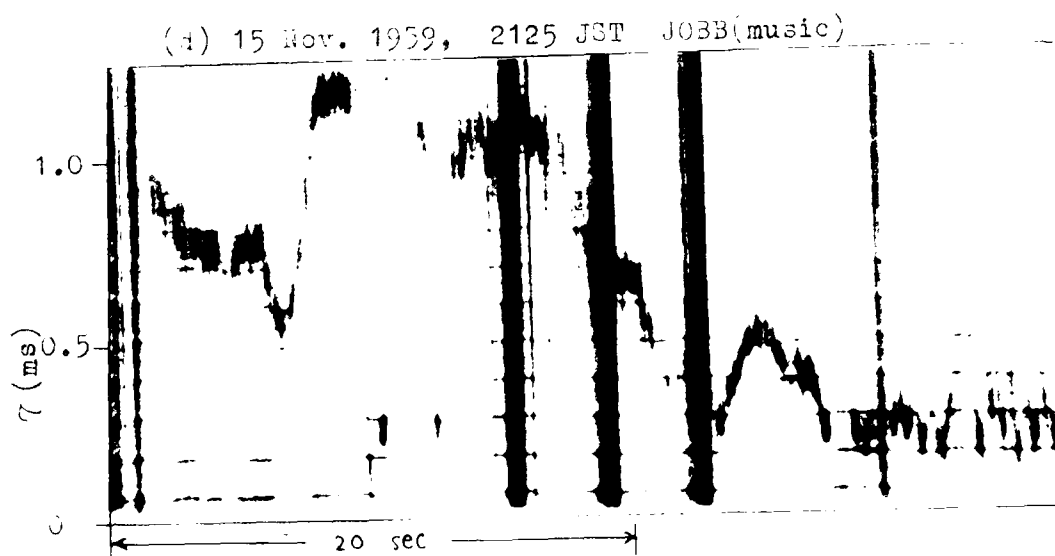
Fig. 3.23(c),(d) records in the Pseudo impulse method (insufficient separation).
