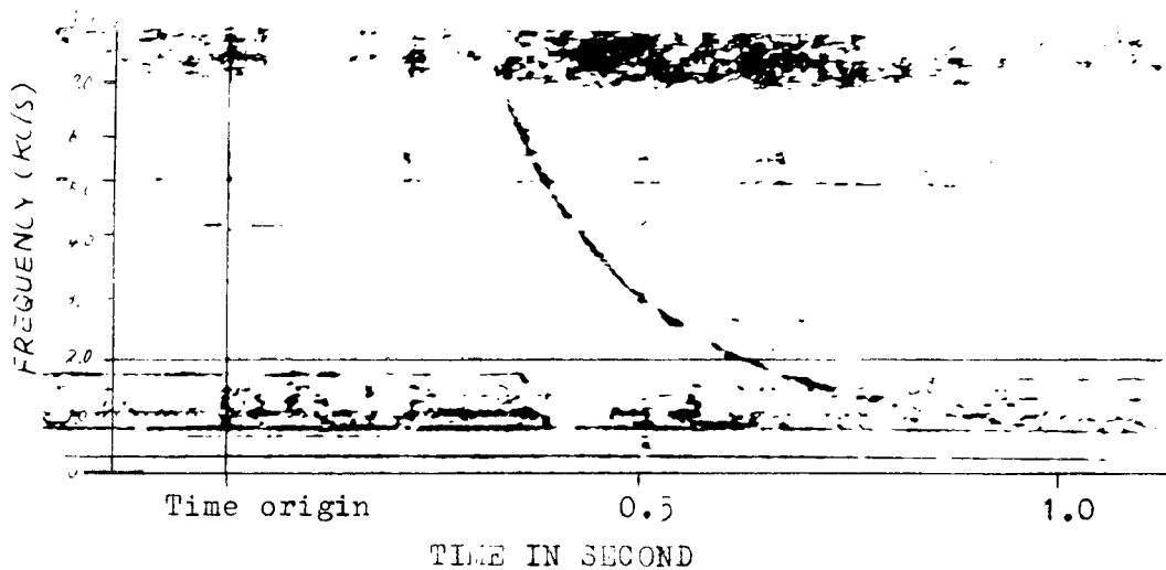
Fig.1.1 An example of the whistler observed at Toyokawa, Japan (After Otsu).
