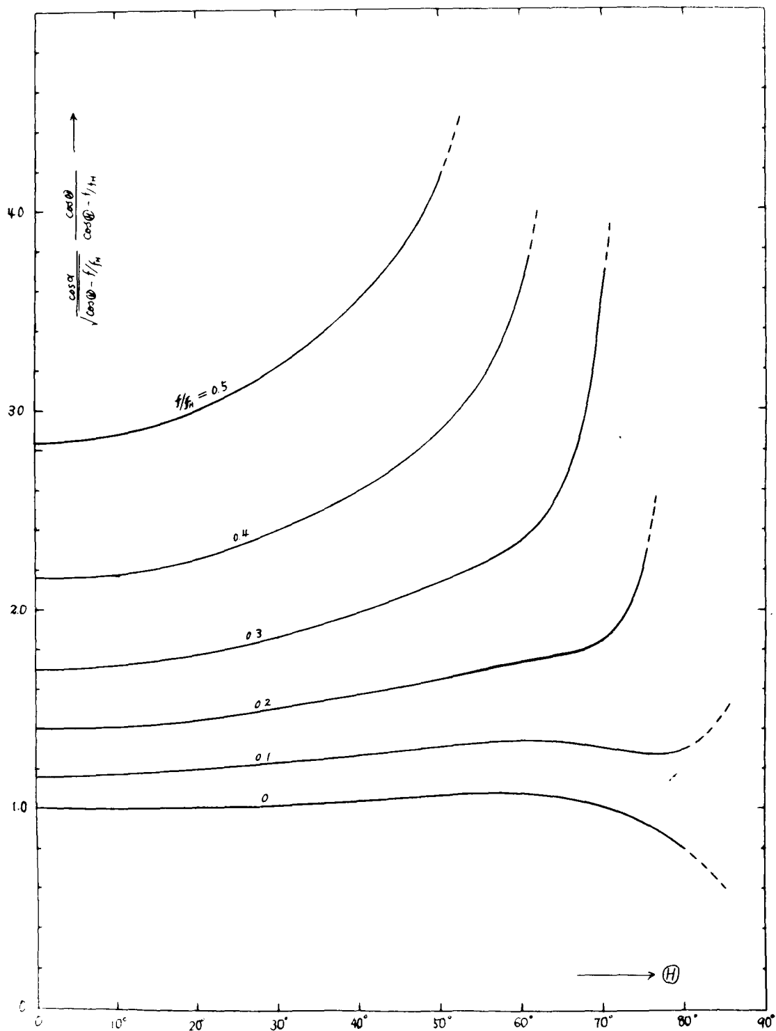
Fig. 1.6 Graph of \frac{\cos \alpha}{\sqrt{\cos \theta - f/f_H}} \cdot \frac{\cos \theta}{\cos \theta - f/f_H} versus \theta , with f/f_H as parameter.
