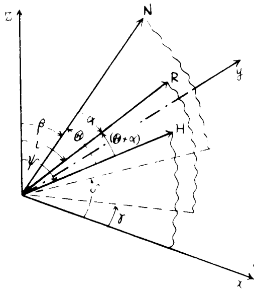
Fig. 1.7 Relation of the directions of magnetic field( H ), wave normal( N ) and ray direction in three dimensional case.
