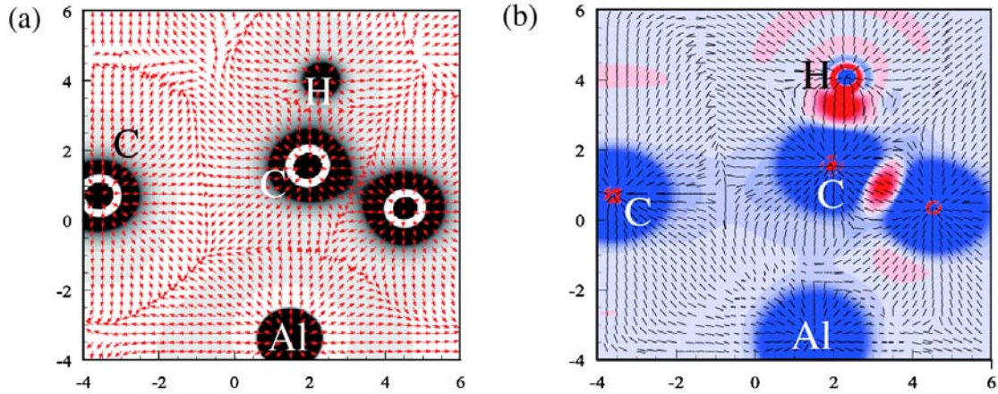
Fig. 7. Electronic energy densities on a cross section of a snapshot in the MD simulation. (a) the positive kinetic energy density in grey region and the tension density in red arrow, and (b) the 3 rd eigenvalue of the stress tensor density in red for positive "tensile" stress, while in blue negative "compressive" stress, and the eigenvector in black line. The axes of ordinate and abscissa are labeled in Bohr.
