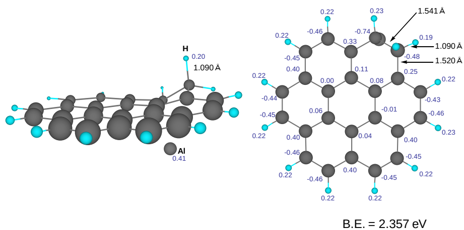
C-site optimized structure
