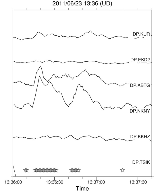
Fig.7 : (a) Preprocessed waveform from 13:36:00 to 13:37:40 (JST) in June 23, 2011. They exhibit clear peaks at stations DP.ABTG and DP.NKNY. Because of the power failure due to the debris flow, DP.TSIK has no data in this time range.
