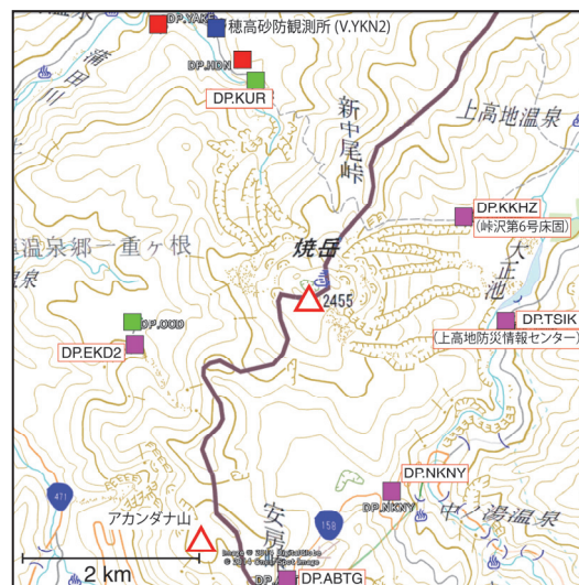
Fig.1 : Distribution of high sensitivity seismic stations. Red, green, and blue squares represent online stations operated by Kyoto Univ., Jindur River System Sabo Office (MLIT), and Japan Meteorological Agency (JMA), respectively. Magenta squares show the offline stations operated by Kyoto Univ.
