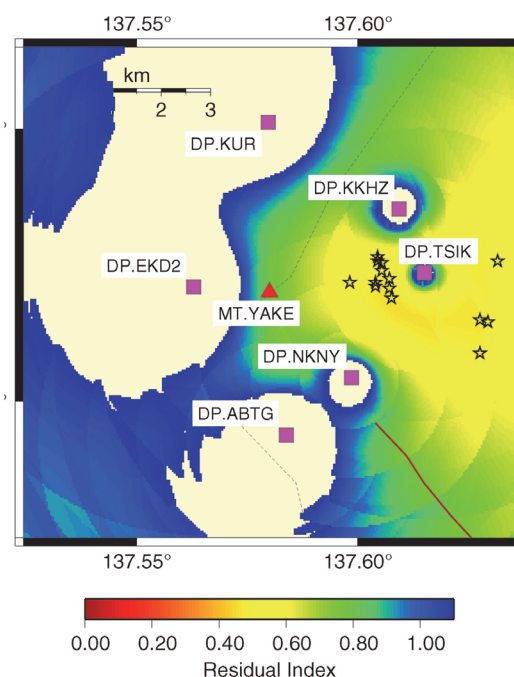
Fig.8 : (b) Estimated location of the seismic source in the time range shown by open stars in Fig.8(a). Open stars in the figure show the seismic sources, however, the estimation error is larger than those in Fig.6(b) and Fig.7(b)
