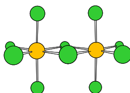
edged-sharing bioctahedral bridged geometry
