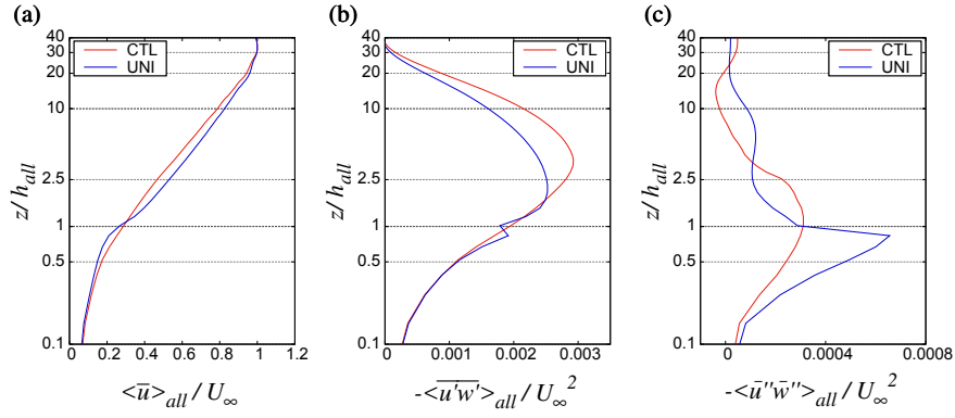
Fig. 8 Vertical profiles of (a) time-averaged streamwise velocity component, (b) Reynolds stress, and (c) dispersive flux averaged spatially over the main region. These values are normalized by U_{\infty} . Red and blue lines denote the result of the CTL and UNI experiments, respectively. The vertical axis is normalized by z = h_{all} . Note that a logarithmic scale is used for the vertical axis.
