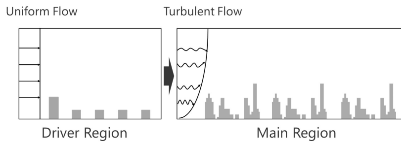
Fig. 4 Schematic of turbulent flows formed in the driver region and imposed on the main region as the inflow condition.
