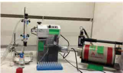
Fig.1. Extraction-chromatography set-up with on-line γ-ray detector for Yb/Lu separation.
