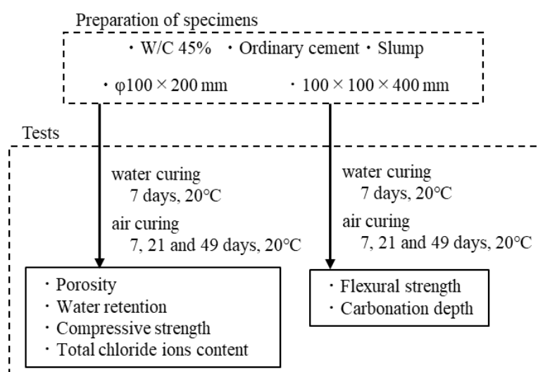
Figure 7.1 Overall flow of this research
