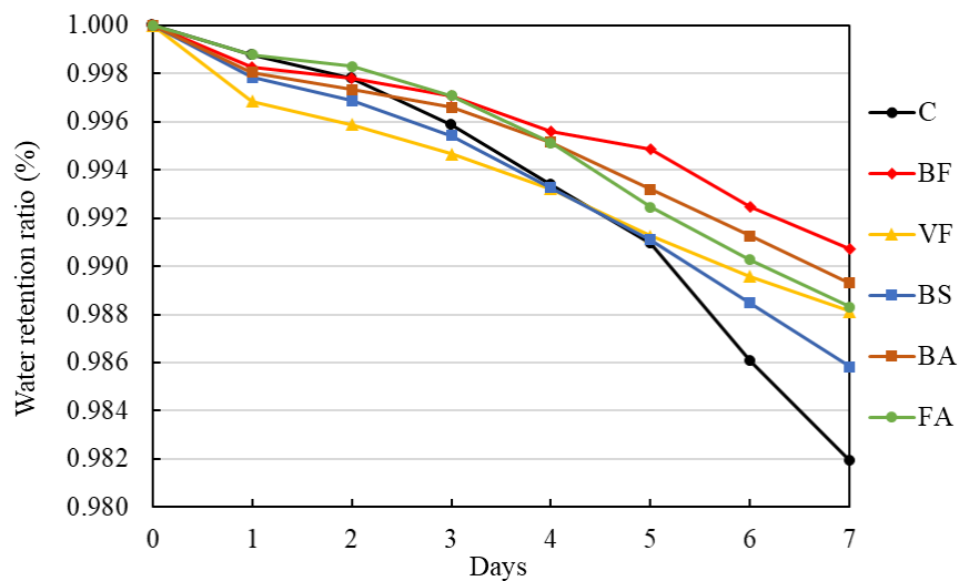
Figure 6.8 Water retention rate of each mixture
