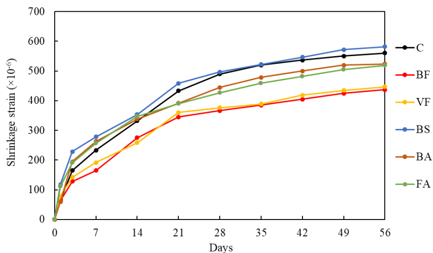
Figure 6.12 Shrinkage strain of shotcrete
