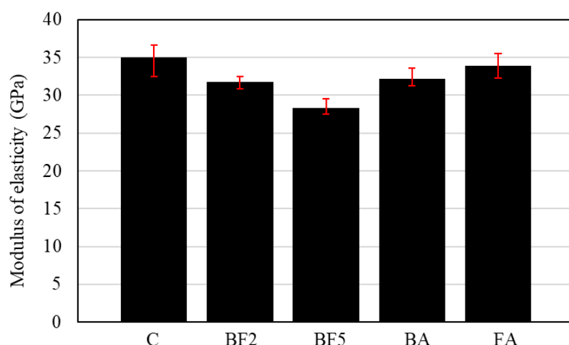
Figure 5.17 Modulus of elasticity of each mixture
