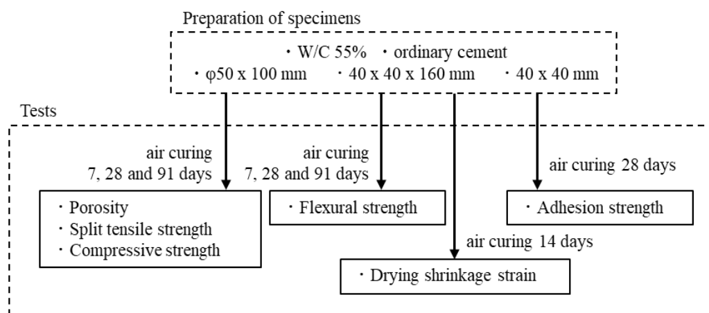
Figure 4.1 Overall flow of this research
