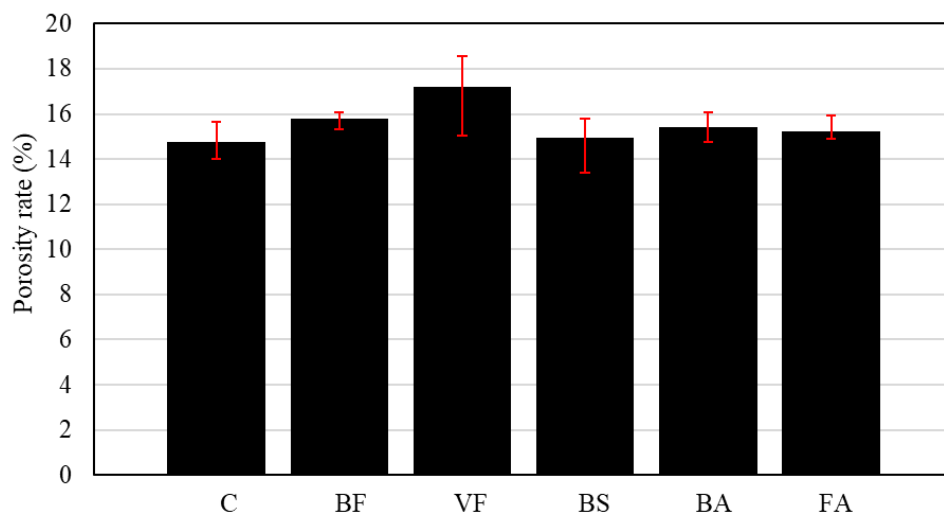
Figure 6.7 Porosity rate of each mixture
