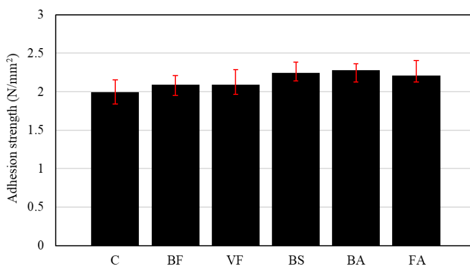
Figure 6.13 Adhesion strength of shotcrete after 28 days of curing
