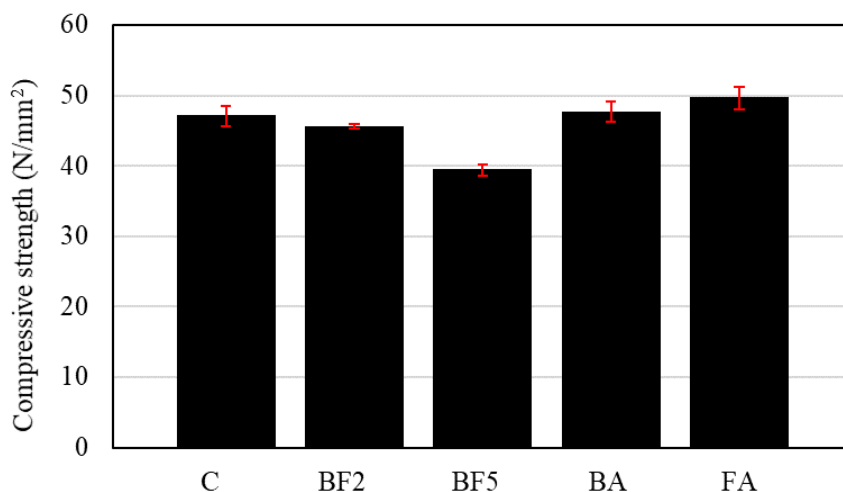
Figure 5.16 Compressive strength of each concrete mixture
