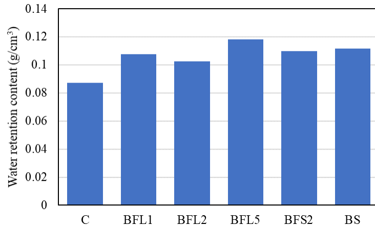
Figure 8.8 Water retention content
