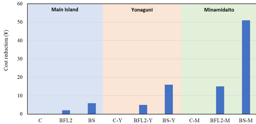
Figure 9.9 Cost reduction associated with the production of interlocking concrete blocks
