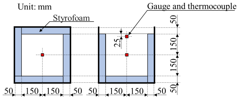
Figure 5.3 Outline of massive concrete specimen
