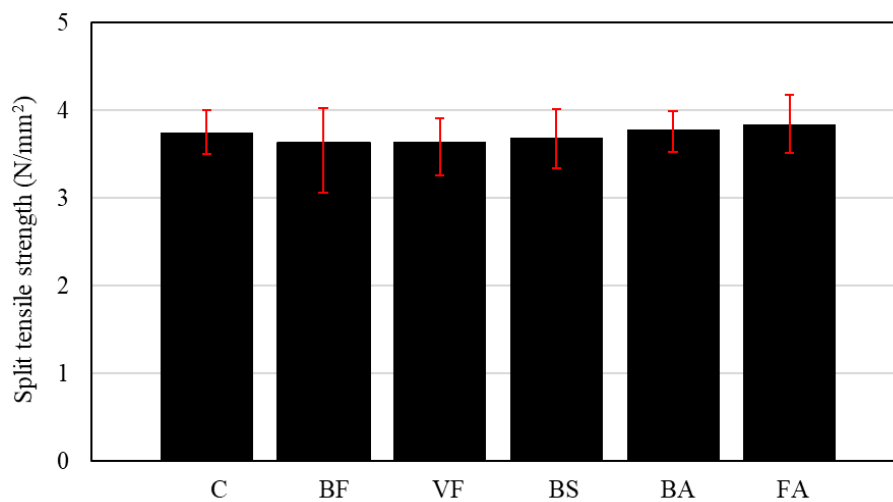
Figure 6.11 Split tensile strength of shotcrete at 28 days
