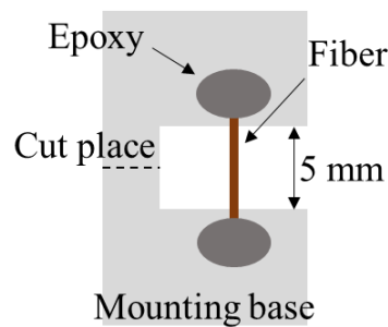
Figure 3.6 Preparation of specimen for the tensile test
