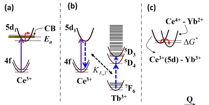
FIG. 4. Schematic illustration of (a) thermal ionization, (b) energy transfer, and (c) electron transfer process (figure not in scale).
