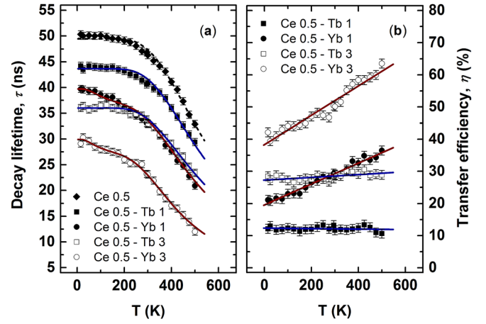
FIG. 3. Temperature dependence on donor luminescence decay lifetimes (a), and transfer efficiency (b). The fits to the experimental data represents theoretical simulations.
