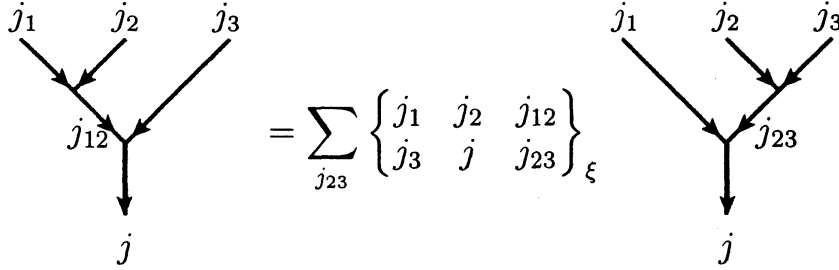
FIGURE 3. The quantum 6j -symbol
