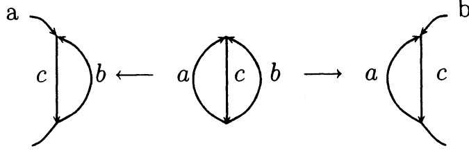
FIGURE 2. On the left \theta_a(a, b, c) ; on the right \theta_b(a, b, c) .
