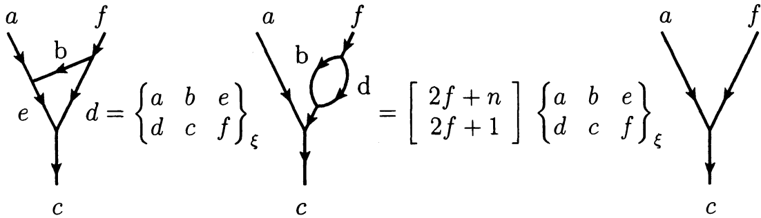
FIGURE 4. Another expression of the quantum 6j -symbol
