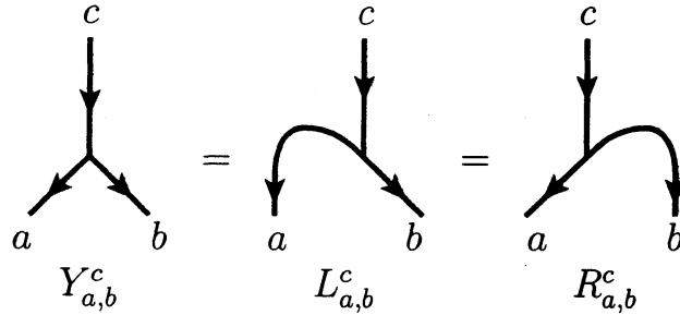
FIGURE 1. The first equality is the definition of Y_{a,b}^c , the second is Lemma 3.4.
