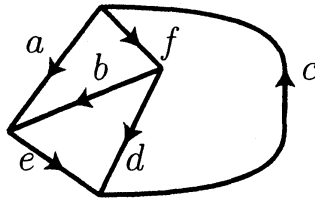
FIGURE 5. Colored oriented tetrahedral graph
