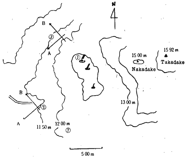
Fig. 2. Positions of the First Crater (1) and observation stations of Hondo (2) and Umanose (3).
