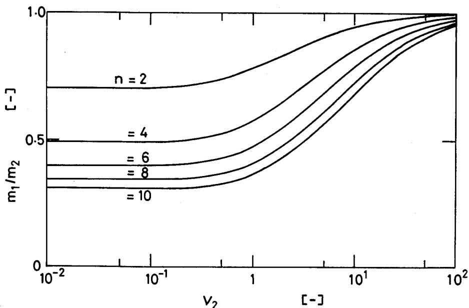
Fig. 8. Relationship between v_2 and m_1/m_2 when C_{A1} = n \cdot C_{A2} ( n > 1 ).
