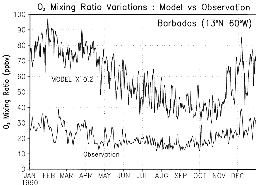
Fig. 4 Comparison of surface ozone variations observed at Barbados (Oltmans and Levy, 1994) with variations in simulated ozone mixing ratio at the adjacent grid point of 60°W longitude, 12.5°N latitude, 850hPa pressure level. Units in ppbv. Note the simulated values are multiplied by 0.2.
