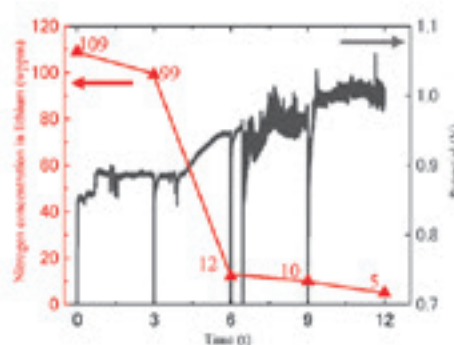
Fig.2 Temporal change of N concentration in liquid Li and the required potential for 2mA current.
